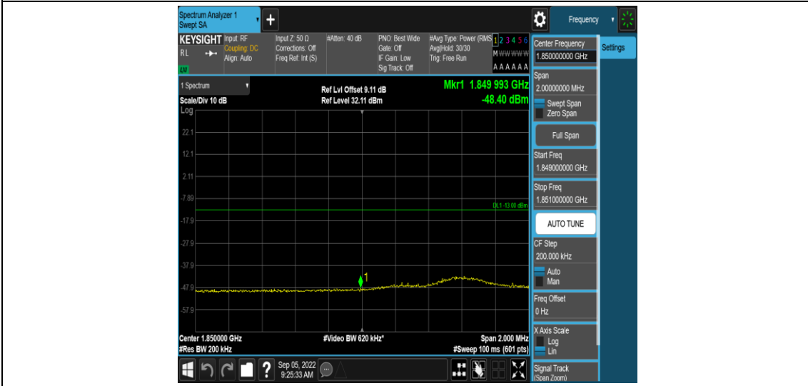
Band2-10MHz-QPSK-18650-1RB#49
