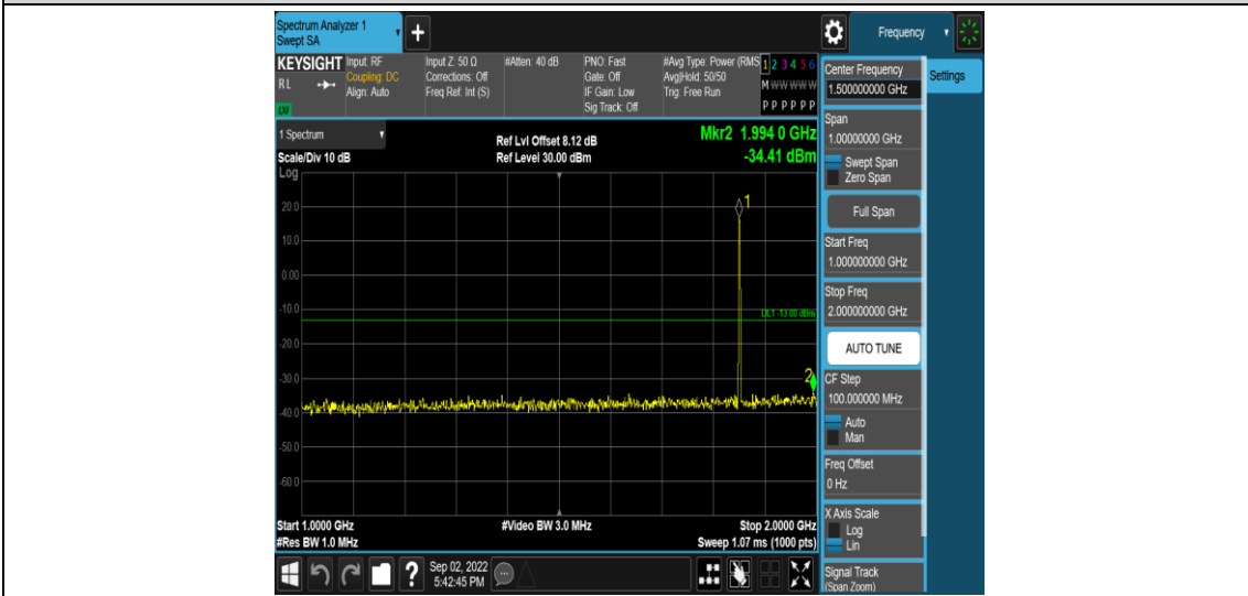
Band2-1.4MHz-QPSK-18607-1RB#0-Range4:1000~2000MHz
