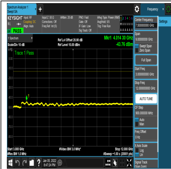
1-N71-PC3-15-20-M-4-DFT-QPSK-Edge_1R B_Left-1@0-3000-12000--43.76--13-PASS
