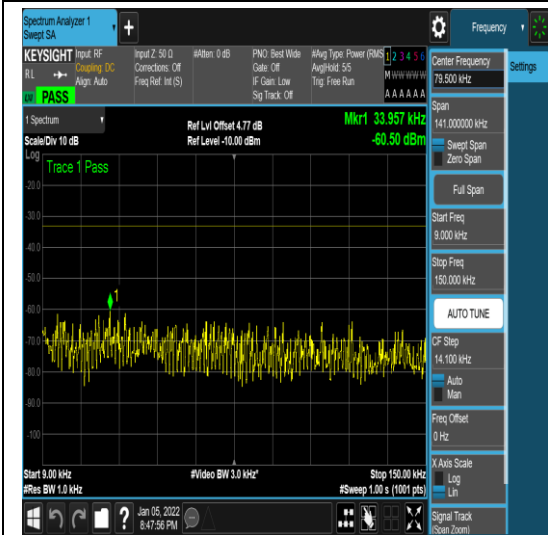
1-N71-PC3-15-20-M-16-CP-QPSK-Edge_1R B_Left-1@0-0.009-0.15--60.50--33-PASS
