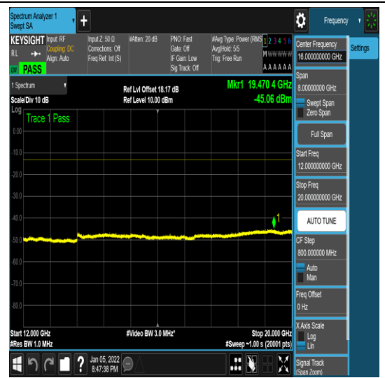
1-N71-PC3-15-20-M-4-DFT-QPSK-Edge_1R B_Left-1@0-12000-20000--45.06--13-PASS
