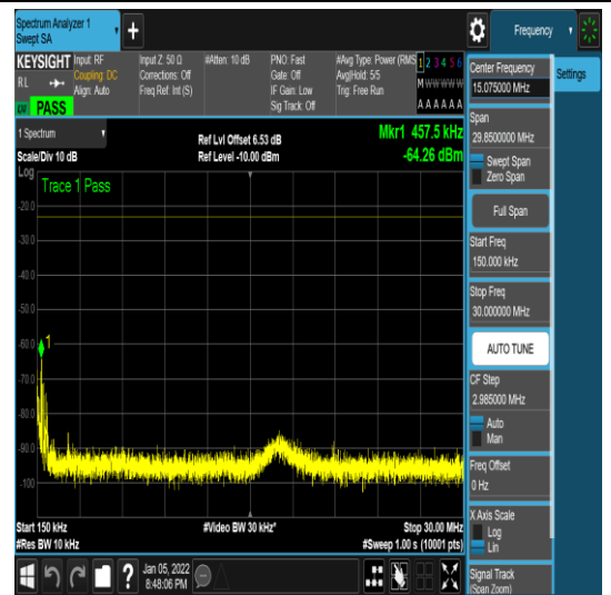
1-N71-PC3-15-20-M-16-CP-QPSK-Edge_1R B_Left-1@0-0.15-30--64.26--23-PASS
