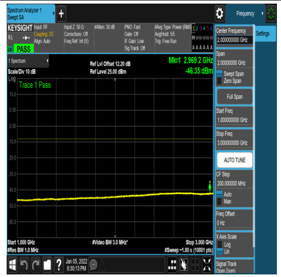
1-N71-PC3-15-10-H-16-CP-QPSK-Edge_1R B_Left-1@0-0.000-0.000--46.35--33-PASS
