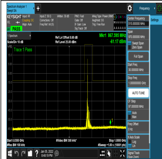
1-N71-PC3-15-20-M-16-CP-QPSK-Edge_1R B_Left-1@0-0.009-0.15--60.50--33-PASS
