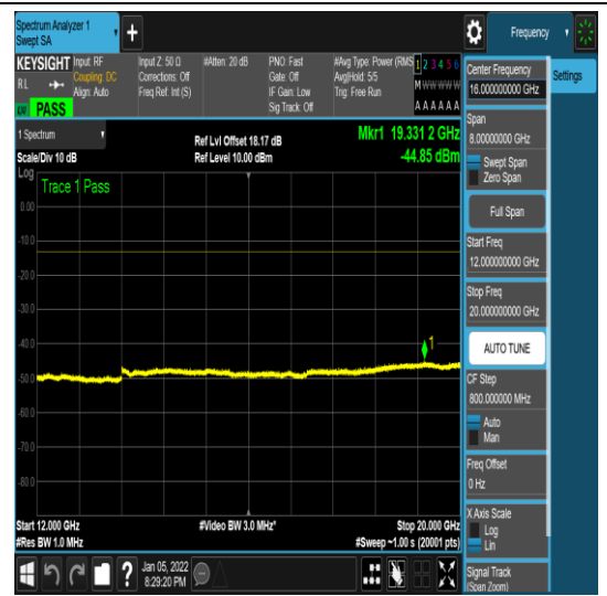
1-N71-PC3-15-10-H-4-DFT-QPSK-Edge_1R B_Left-1@0-12000-20000--44.85--13-PASS
