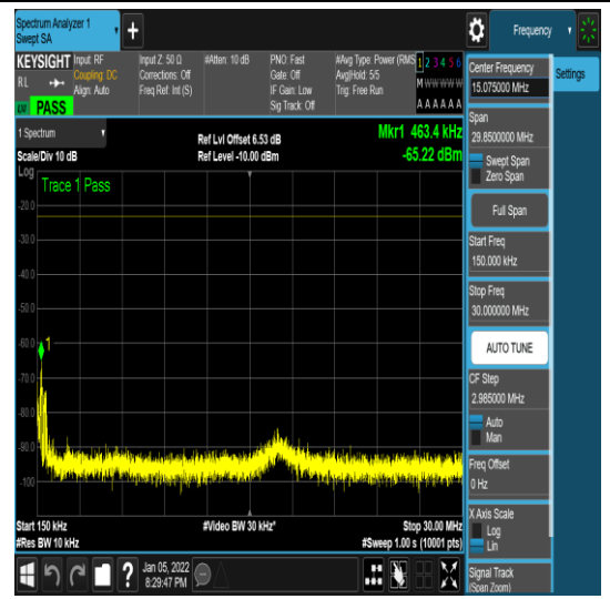
1-N71-PC3-15-10-H-16-CP-QPSK-Edge_1R B_Left-1@0-0.15-30--65.22--23-PASS
