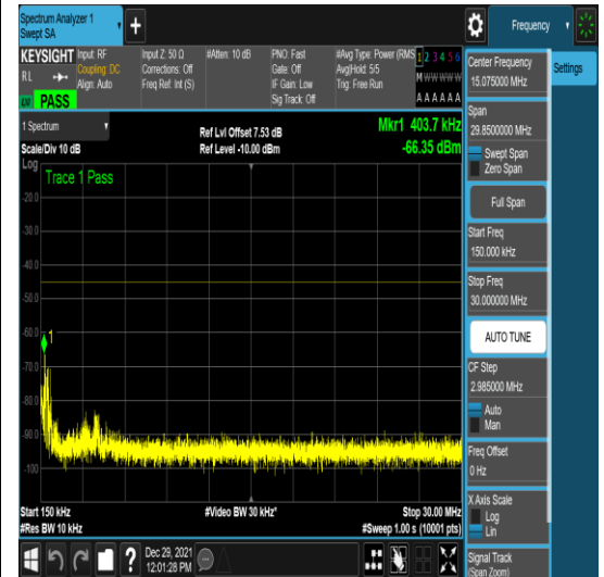
n41-PC3-30-60-L-4-N/A-N/A-N/A-DFT-QPSK -Edge_1RB_Left-1@0-0.15-30--66.35--45-PA SS
