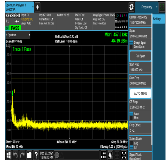
n41-PC3-30-60-H-4-N/A-N/A-N/A-DFT-QPSK -Edge_1RB_Left-1@0-0.15-30--64.19--45-PA SS
