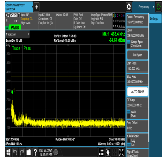
n41-PC3-30-90-H-4-N/A-N/A-N/A-DFT-QPSK -Edge_1RB_Left-1 @0-0.15-30--64.67--45-PA SS
