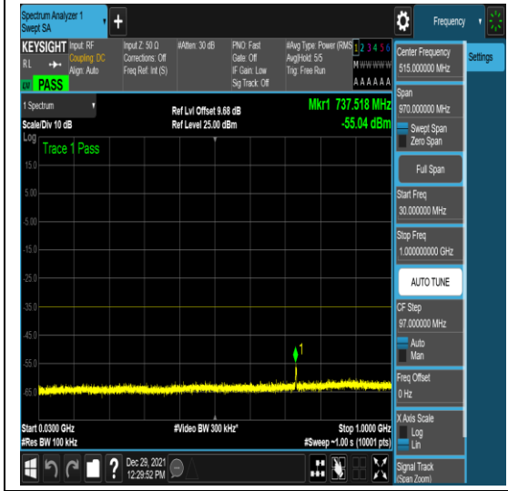
n41-PC3-30-90-M-16-N/A-N/A-N/A-CP-QPS K-Edge_1RB_Left-1@0-30-1000--55.04--35- PASS
