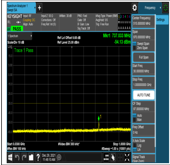
n41-PC3-30-40-H-16-N/A-N/A-N/A-CP-QPSK -Edge_1RB_Left-1@0-30-1000--54.13--35-P ASS
