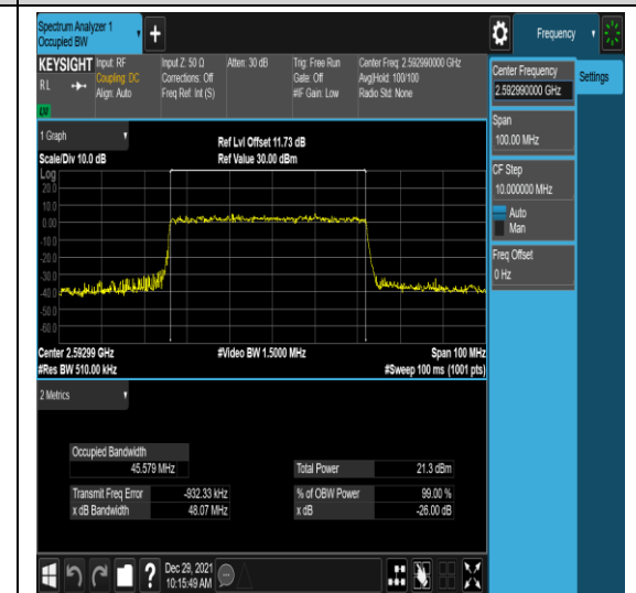
n41-PC3-30-50-M-4-N/A-N/A-N/A-DFT-64QA M-Outer_Full-128@0-Ant1-45.579-48.07-≤50 -PASS
