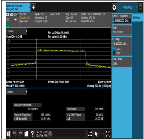
n41-PC3-30-80-H-7-N/A-N/A-N/A-CP-64QA M-Outer_Full-217@0-Ant1-77.256-80.14-≤80 -PASS
