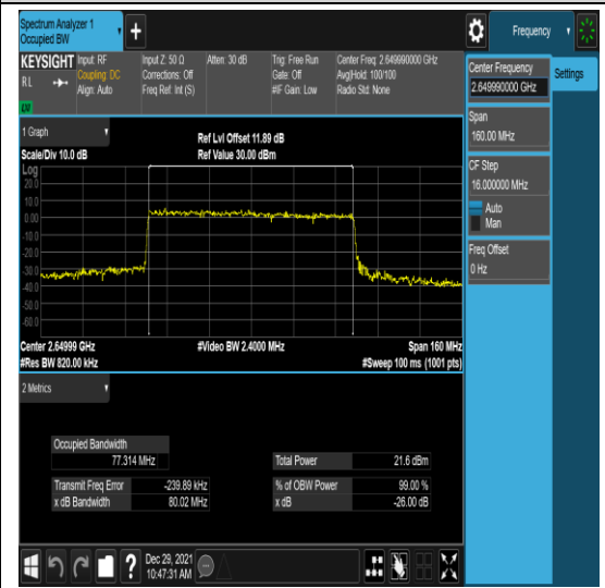
n41-PC3-30-80-H-8-N/A-N/A-N/A-CP-256QA M-Outer_Full-217@0-Ant1-77.314-80.02-≤80 -PASS
