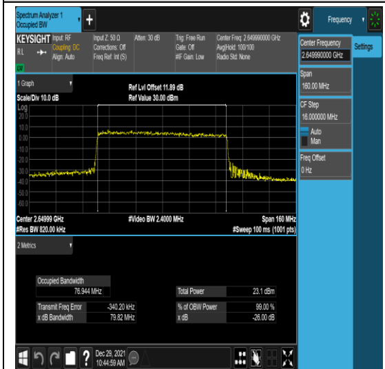
n41-PC3-30-80-H-3-N/A-N/A-N/A-DFT-16QA M-Outer_Full-216@0-Ant1-76.944-79.82-≤80 -PASS
