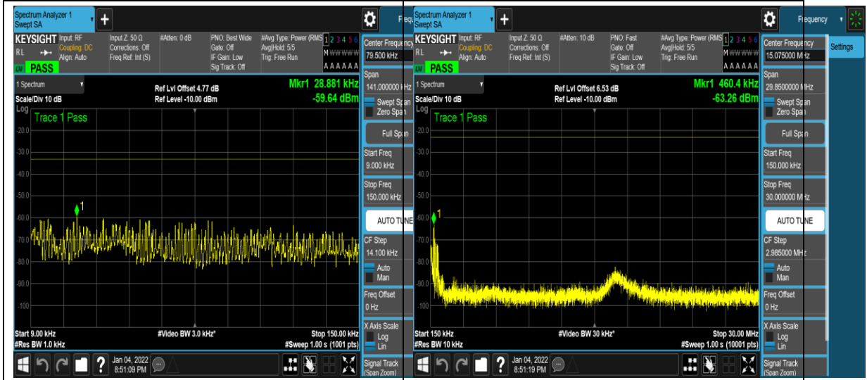
1-N5-PC3-15-20-M-16-CP-QPSK-Edge_1RB _Left-1 @0-0.009-0.15--59.64--33-PASS 1-N5-PC3-15-20-M-16-CP-QPSK-Edge_1RB _Left-1 @0-0.15-30--63.26--23-PASS
