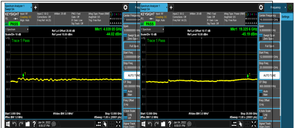
1-N5-PC3-15-20-M-4-DFT-QPSK-Edge_1RB _Left-1 @0-3000-12000--44.02--13-PASS 1-N5-PC3-15-20-M-4-DFT-QPSK-Edge_1RB _Left-1 @0-12000-20000--45.19--13-PASS
