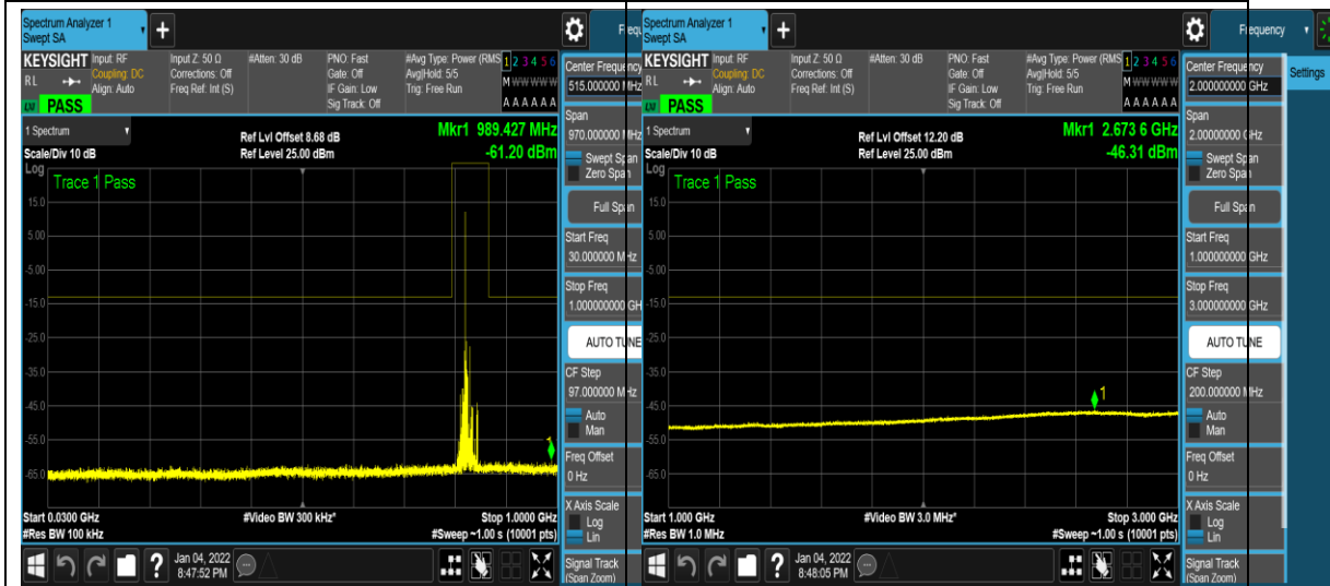
1-N5-PC3-15-20-L-16-CP-QPSK-Edge_1RB _Left-1 @ 0-30-1000--61.20--13-PASS
