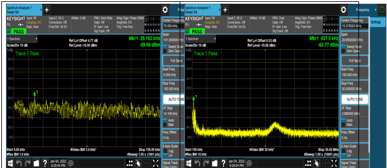
1-N5-PC3-15-10-M-16-CP-QPSK-Edge_1RB _Left-1 @ 0-0.009-0.15--59.06--33-PASS
