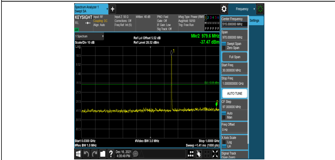
Band71-5MHz-16QAM-133147-1RB#0-Range3:30~1000MHz
