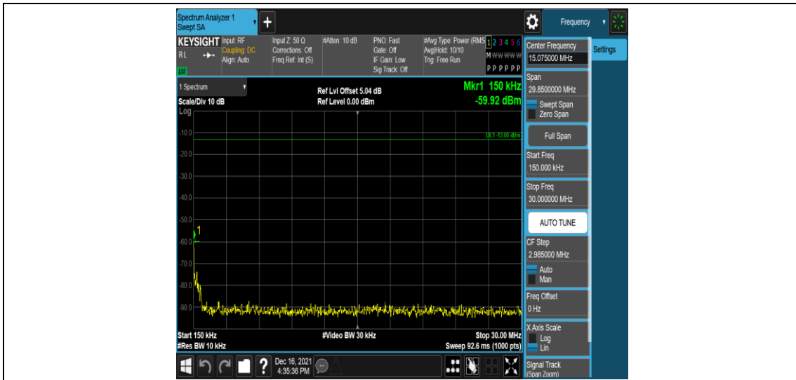
Band71-5MHz-16QAM-133147-1RB#0-Range2:0.15~30MHz
