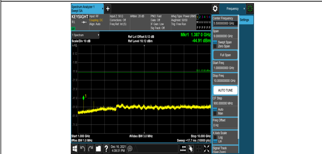
Band71-5MHz-16QAM-133447-1RB#0-Range4:1000~10000MHz
