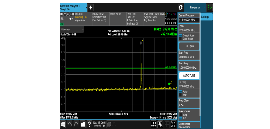
Band71-10MHz-QPSK-133422-1RB#0-Range3:30~1000MHz
