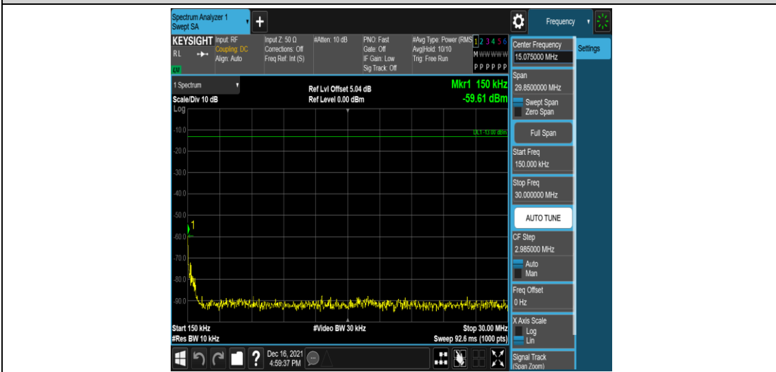
Band71-10MHz-16QAM-133422-1RB#0-Range2:0.15~30MHz
