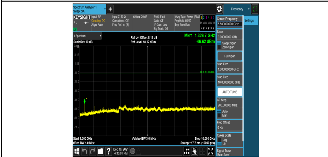
Band71-5MHz-16QAM-133147-1RB#0-Range4:1000~10000MHz
