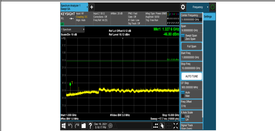
Band71-15MHz-QPSK-133197-1RB#0-Range4: 1000~10000MHz
