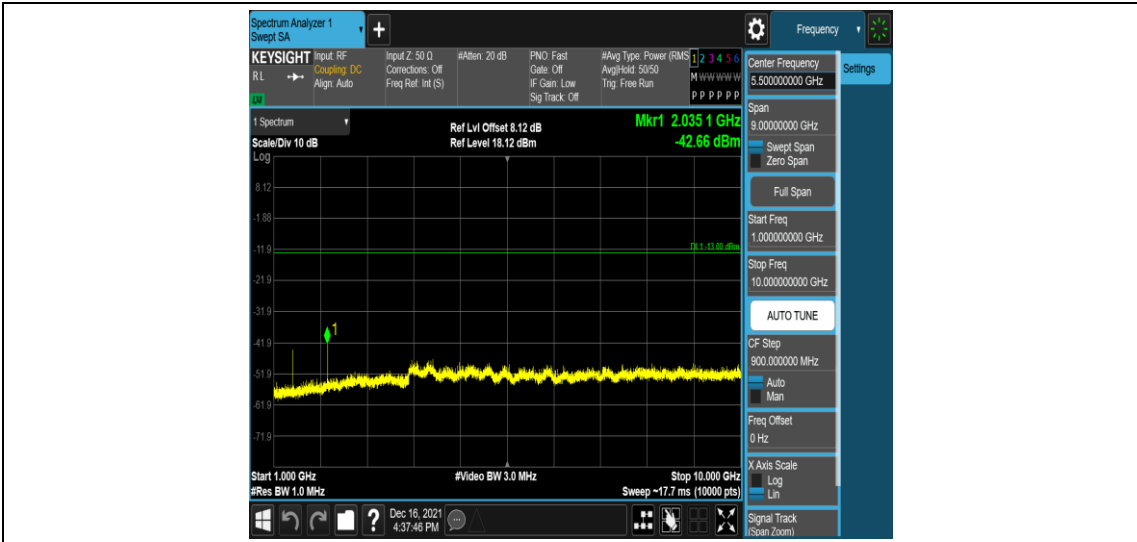
Band71-5MHz-16QAM-133297-1RB#0-Range4: 1000~10000MHz
