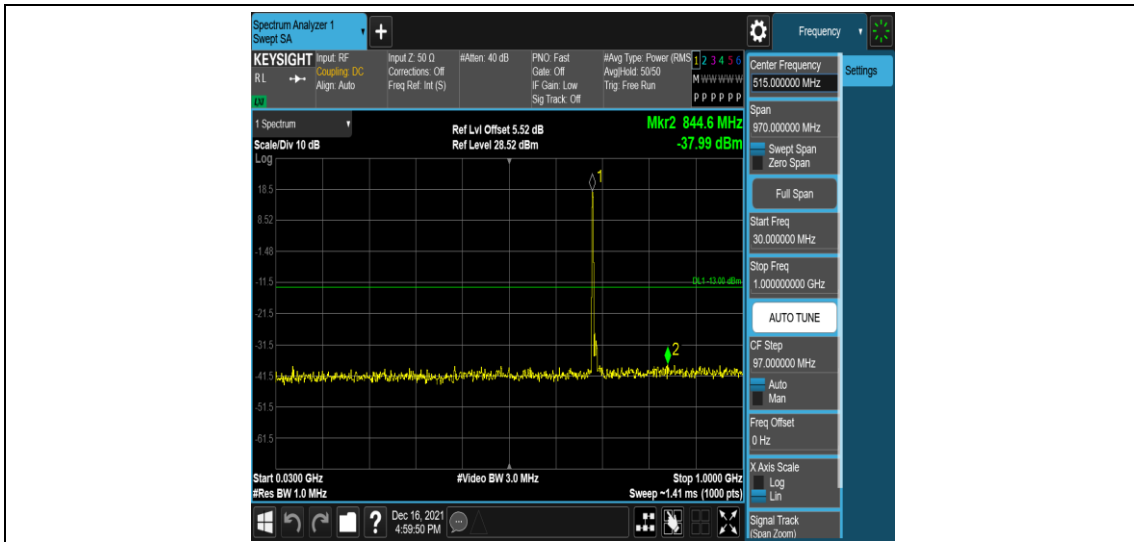
Band71-10MHz-16QAM-133422-1RB#0-Range3:30~1000MHz
