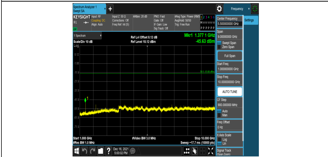
Band71-10MHz-16QAM-133422-1RB#0-Range4:1000~10000MHz
