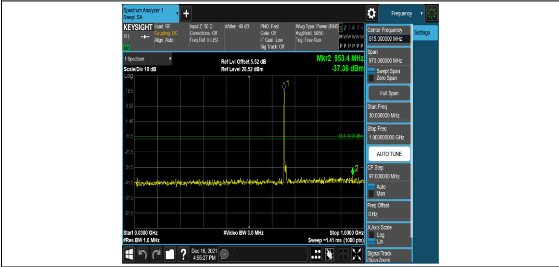
Band71-10MHz-QPSK-133172-1RB#0-Range3:30~1000MHz
