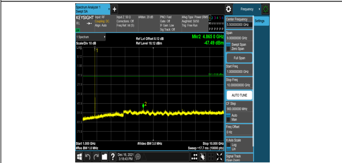
Band66-5MHz-16QAM-132647-1RB#0-Range4:1000~10000MHz
