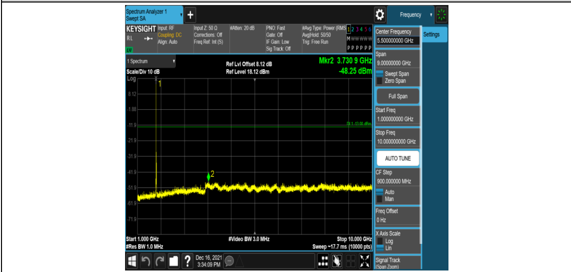
Band66-10MHz-QPSK-132022-1RB#0-Range4: 1000~10000MHz
