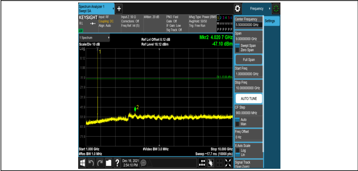
Band66-3MHz-QPSK-131987-1RB#0-Range4:1000~10000MHz
