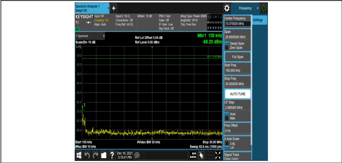
Band66-5MHz-QPSK-132322-1RB#0-Range2:0.15~30MHz
