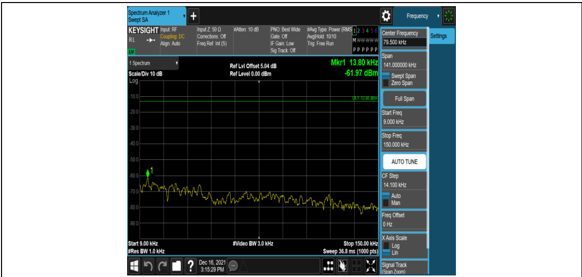
Band66-5MHz-QPSK-132322-1RB#0-Range1:0.009~0.15MHz
