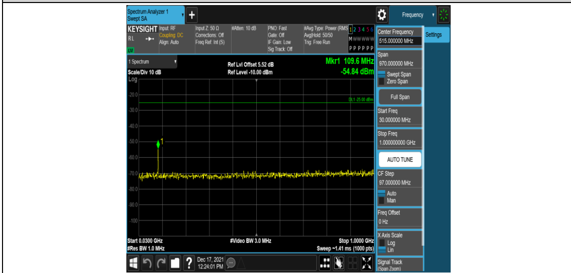
Band41-20MHz-QPSK-41490-1RB#0-Range3:30~1000MHz
