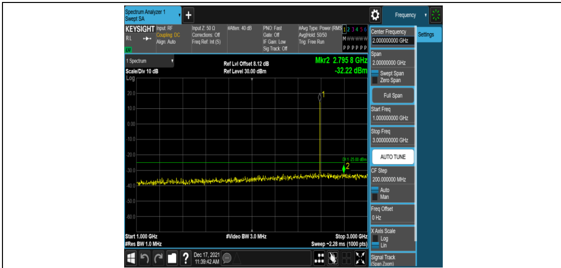
Band41-10MHz-16QAM-40620-1RB#0-Range4:1000~3000MHz
