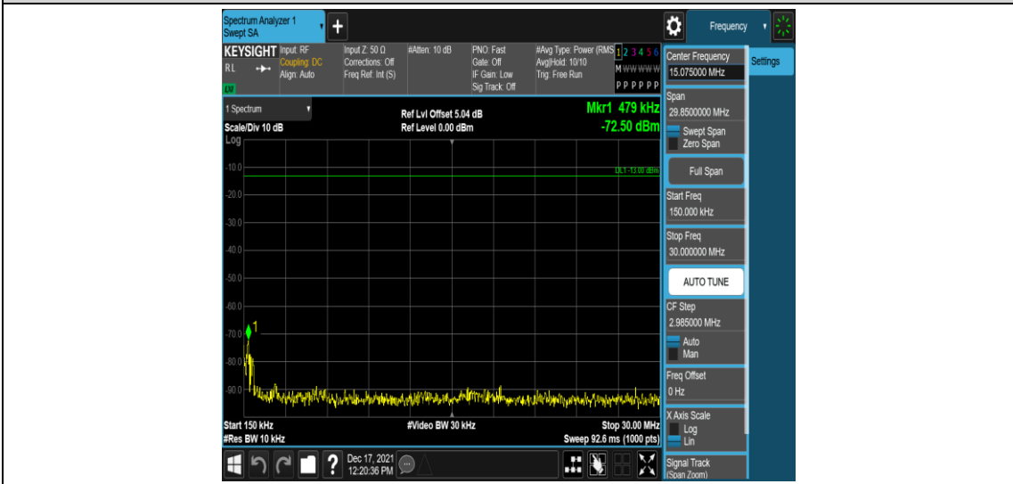
Band41-20MHz-16QAM-39750-1RB#0-Range2:0.15~30MHz
