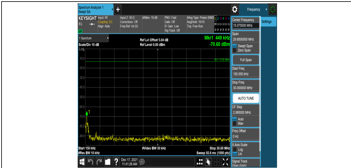
Band41-10MHz-16QAM-41540-1RB#0-Range2:0.15~30MHz
