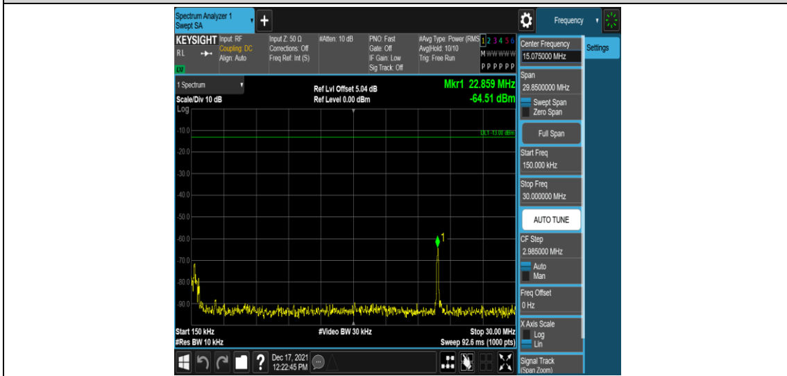
Band41-20MHz-16QAM-40620-1RB#0-Range2:0.15~30MHz
