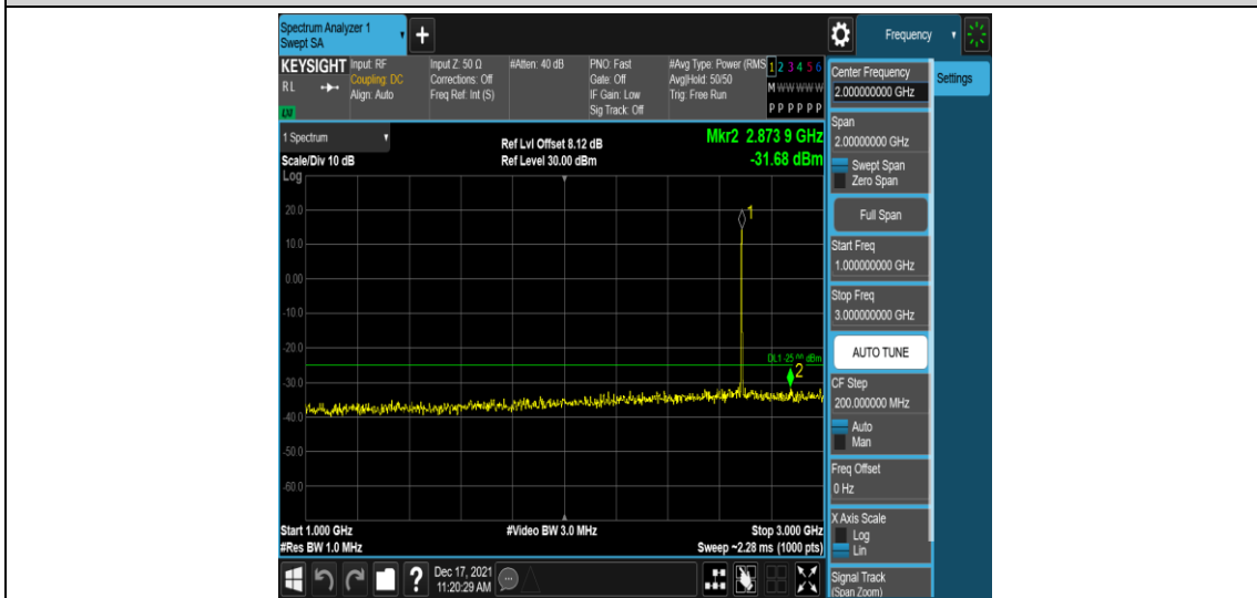
Band41-5MHz-16QAM-41565-1RB#0-Range4:1000~3000MHz
