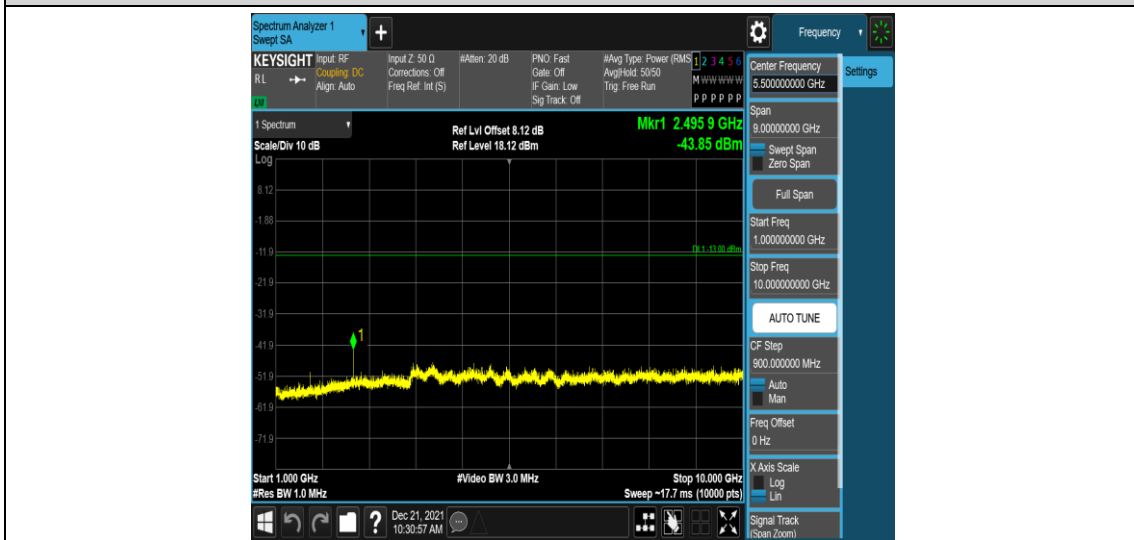
Band26-10MHz-QPSK-26915-1RB#0-Range4:1000~10000MHz
