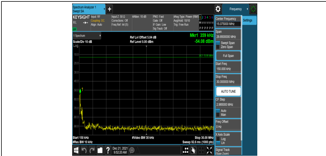
Band26-3MHz-16QAM-26915-1RB#0-Range2:0.15~30MHz
