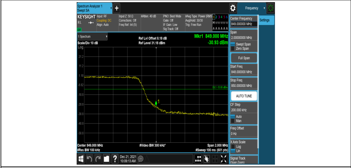
Band26-5MHz-16QAM-27015-25RB#0
