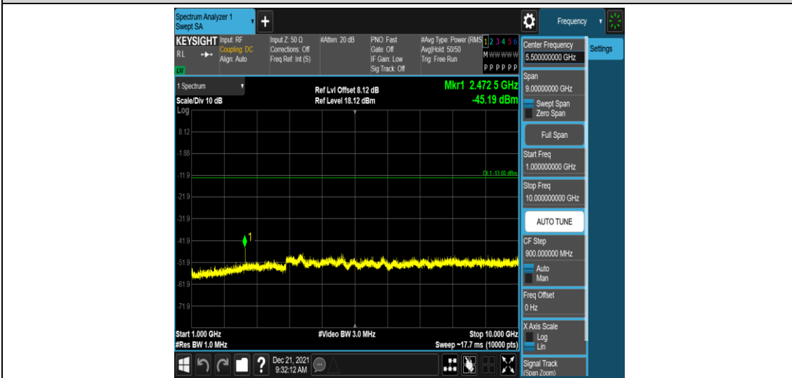
Band26-1.4MHz-16QAM-26797-1RB#0-Range4:1000~10000MHz
