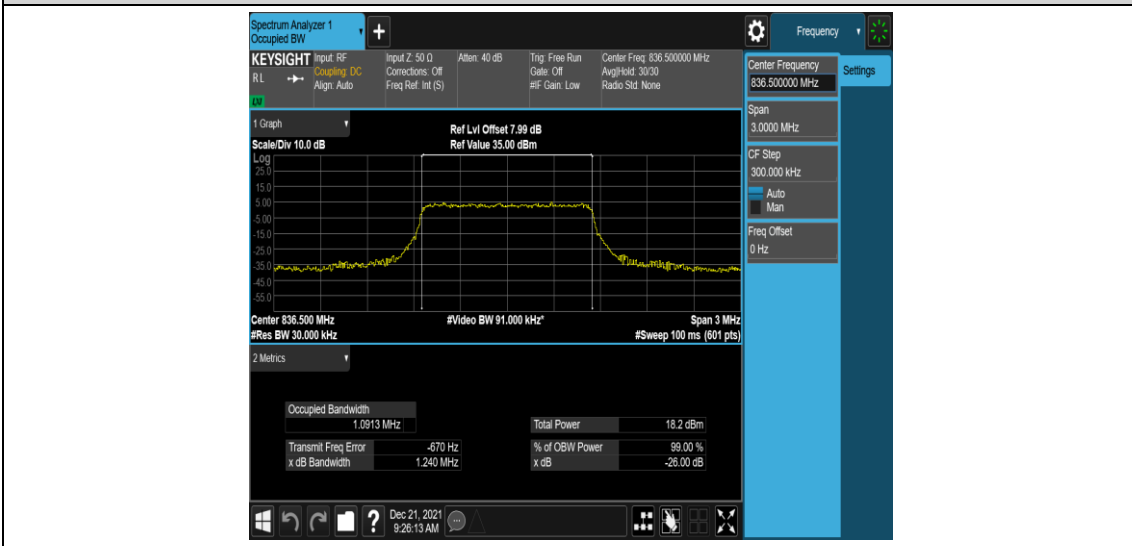
Band26-1.4MHz-QPSK-26915-6RB#0
