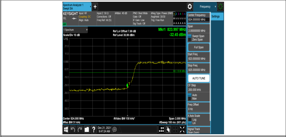
Band26-3MHz-16QAM-26805-15RB#0
