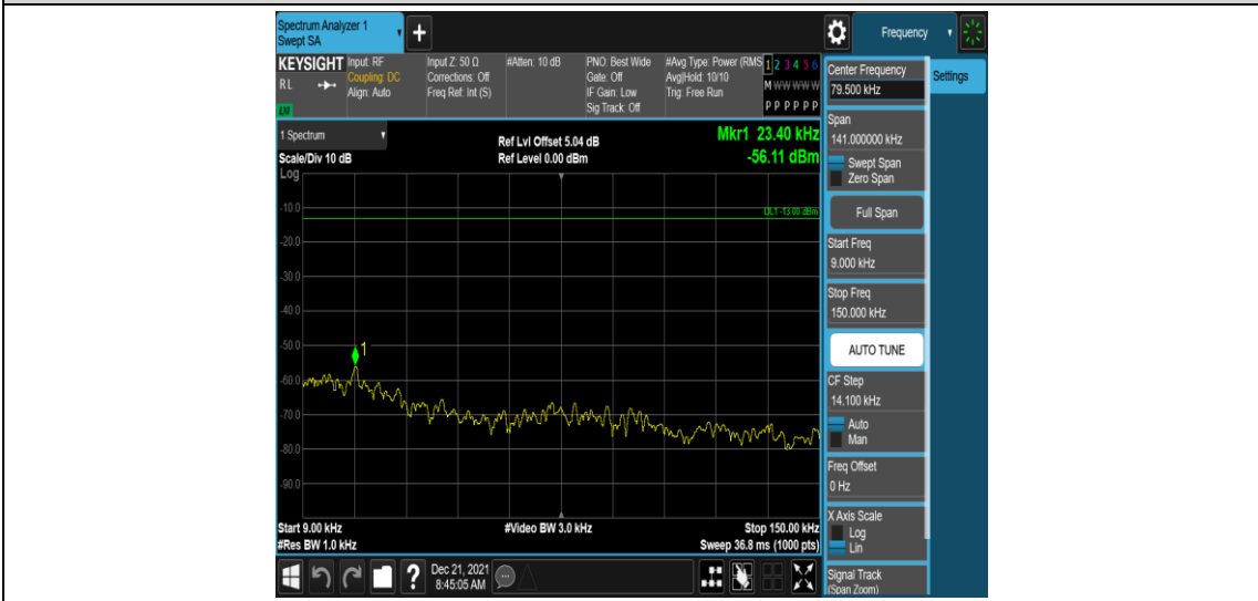
Band26-5MHz-16QAM-26740-1RB#0-Range1:0.009~0.15MHz
