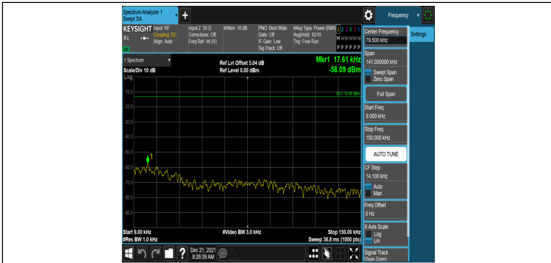
Band26-3MHz-QPSK-26775-1RB#0-Range1:0.009~0.15MHz
