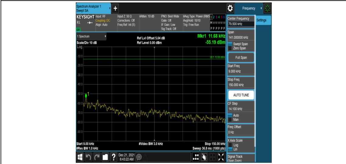
Band26-5MHz-16QAM-26715-1RB#0-Range1:0.009~0.15MHz
