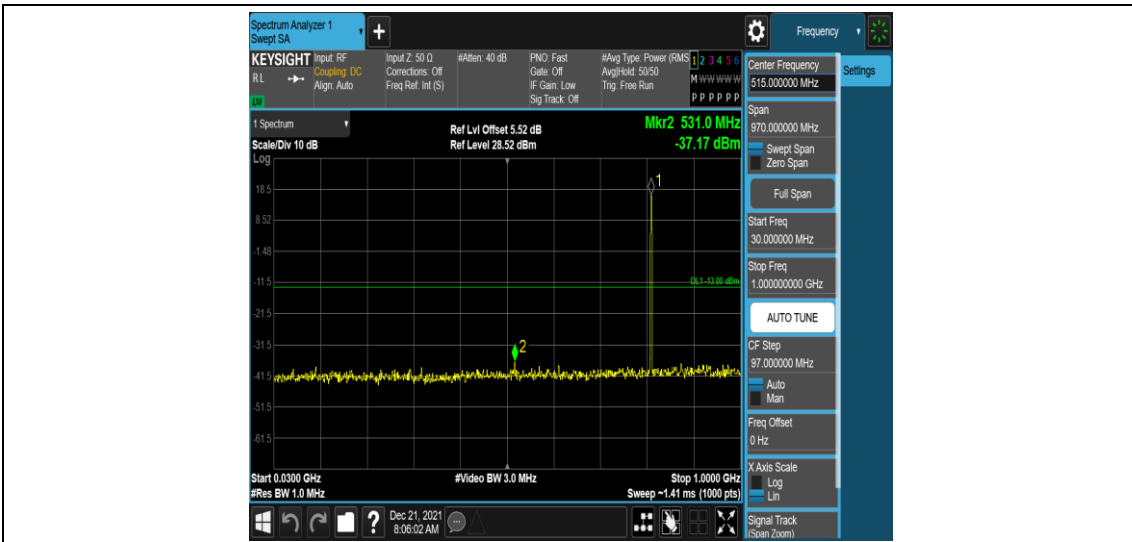
Band26-1.4MHz-16QAM-26697-1RB#0-Range3:30~1000MHz
