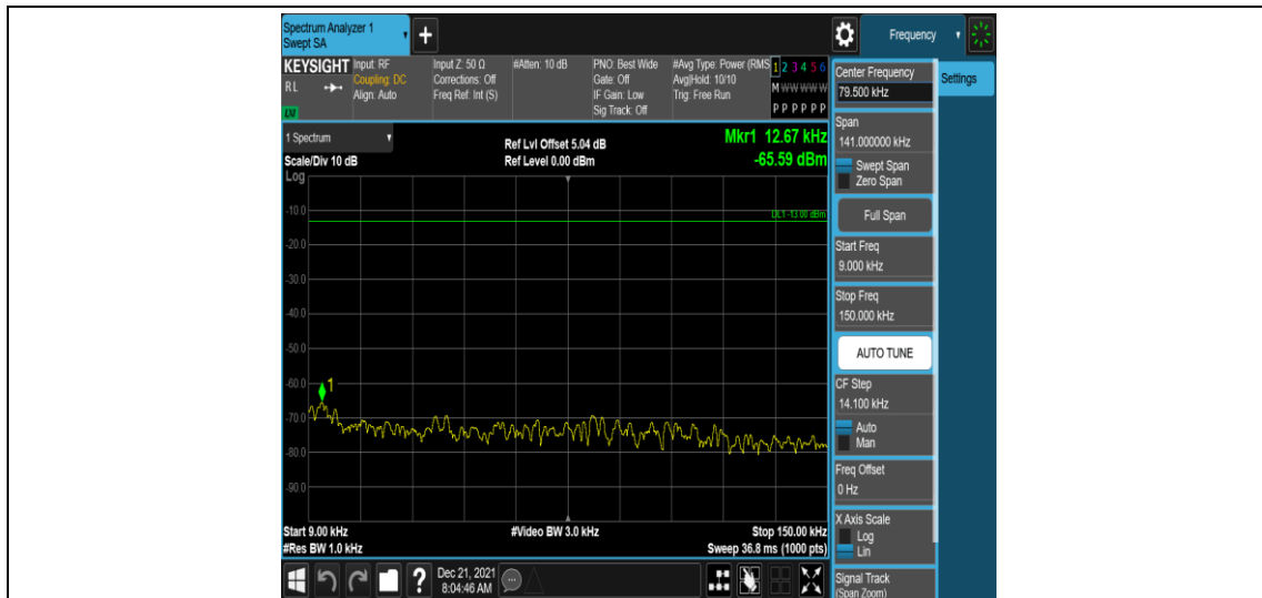
Band26-1.4MHz-QPSK-26697-1RB#0-Range1:0.009~0.15MHz
