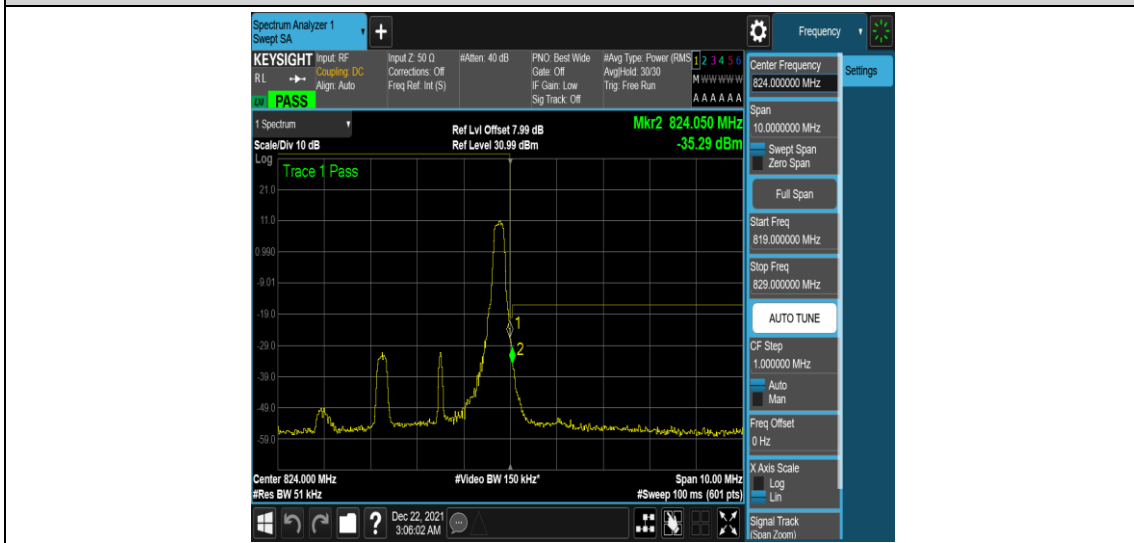
Band26-3MHz-16QAM-26775-1RB#14
