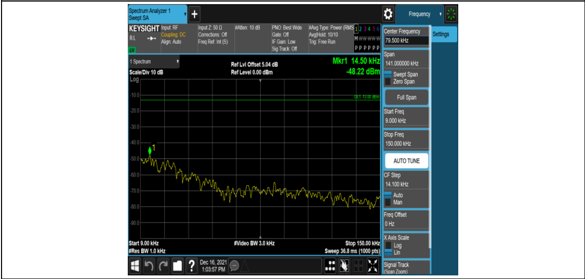
Band25-20MHz-QPSK-26365-1RB#0-Range1:0.009~0.15MHz
