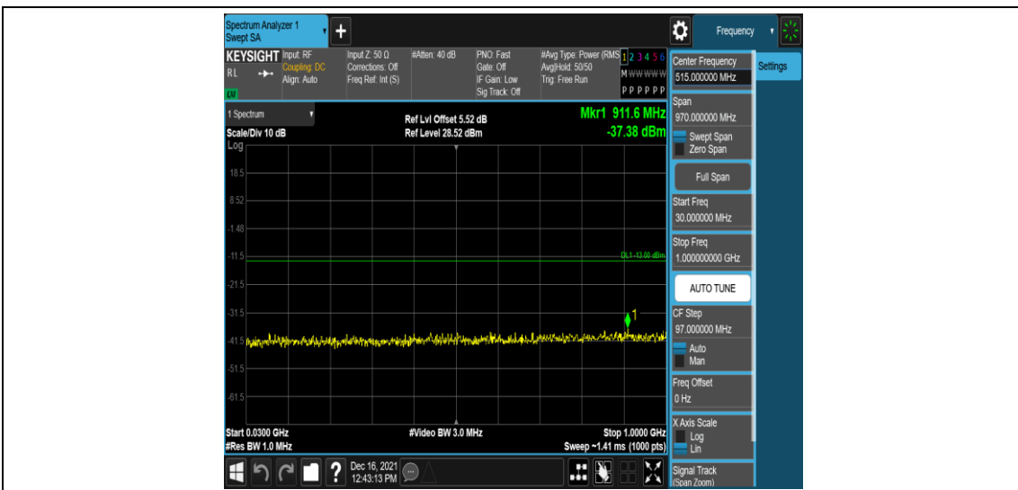
Band25-15MHz-QPSK-26365-1RB#0-Range3:30~1000MHz
