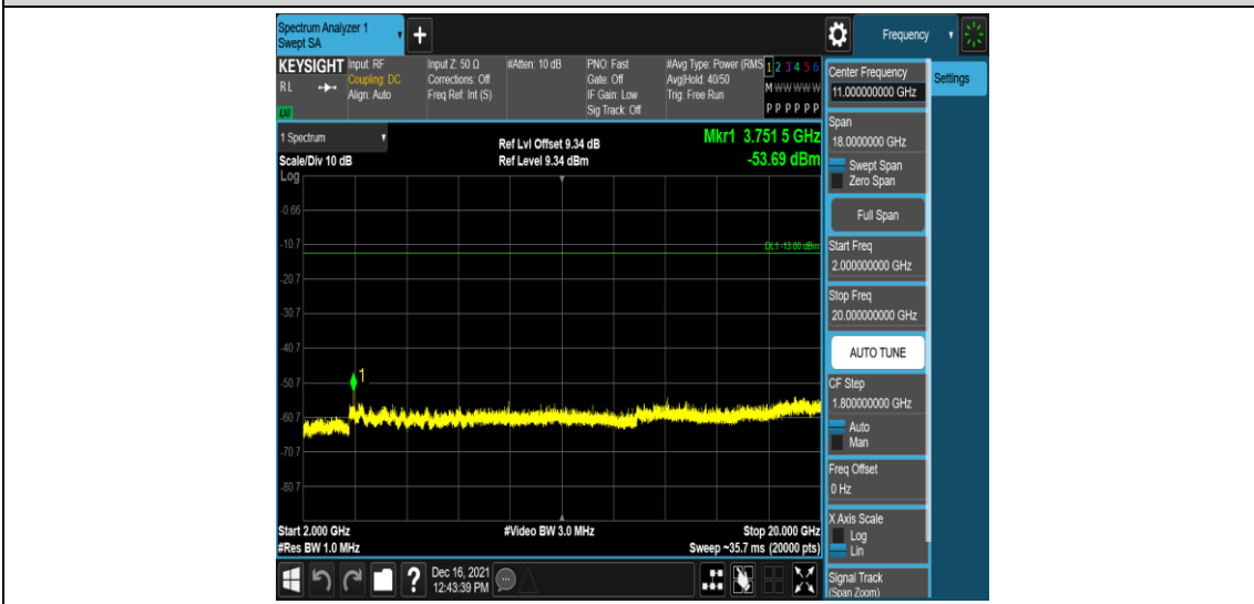
Band25-15MHz-QPSK-26365-1RB#0-Range5:2000~20000MHz
