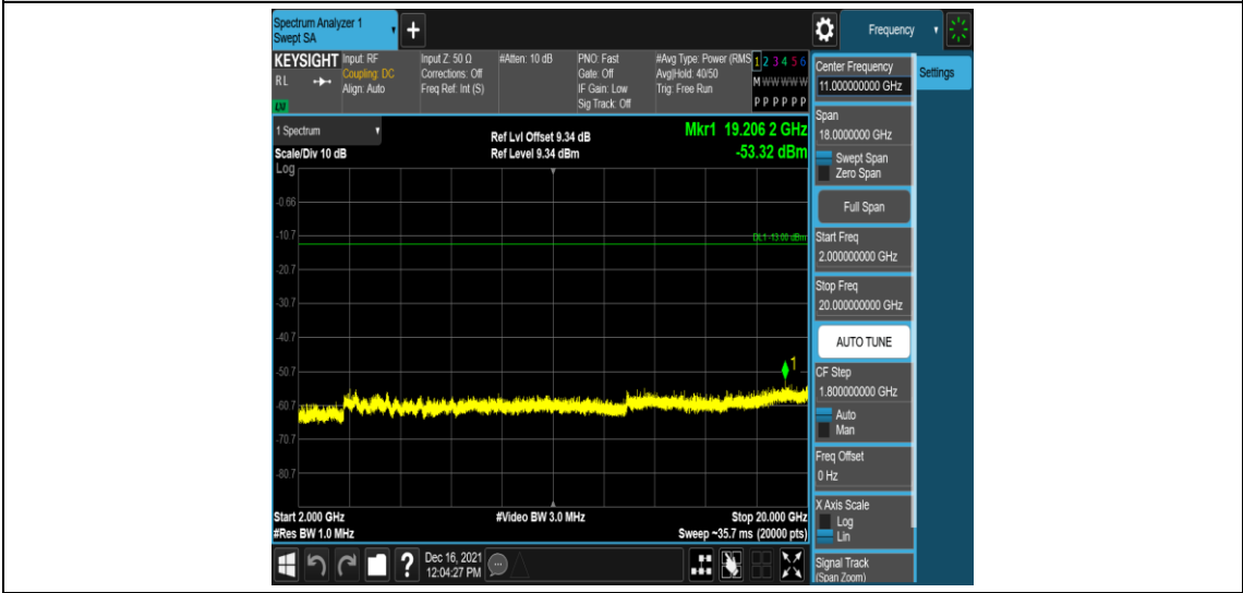
Band25-5MHz-QPSK-26665-1RB#0-Range5:2000~20000MHz
