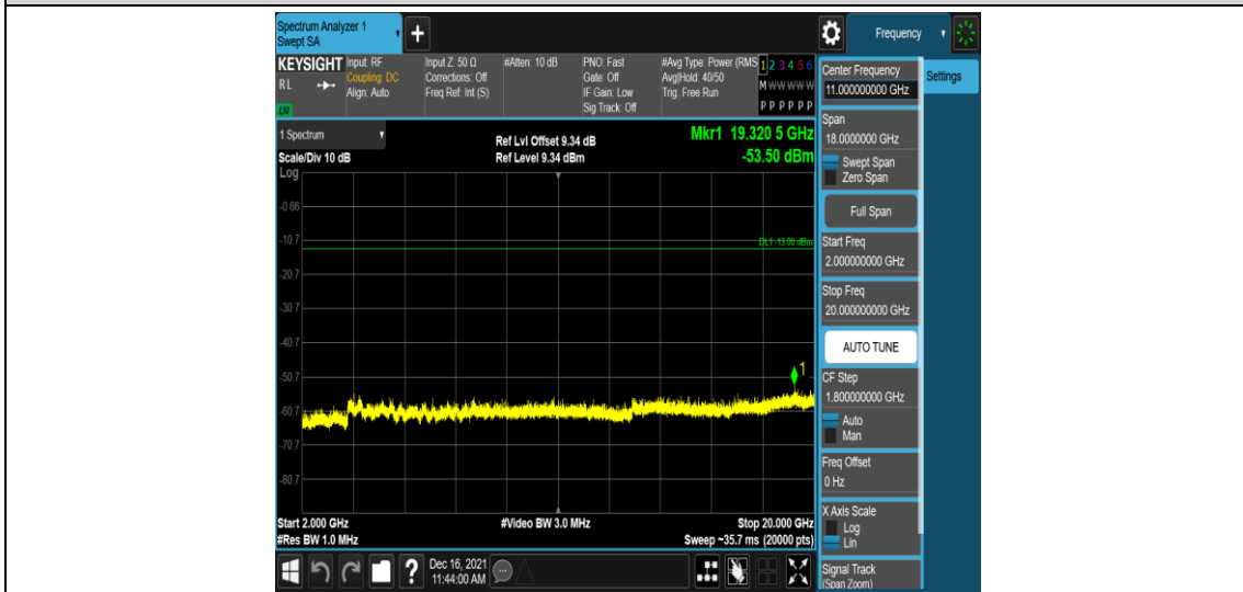
Band25-3MHz-16QAM-26675-1RB#0-Range5:2000~20000MHz
