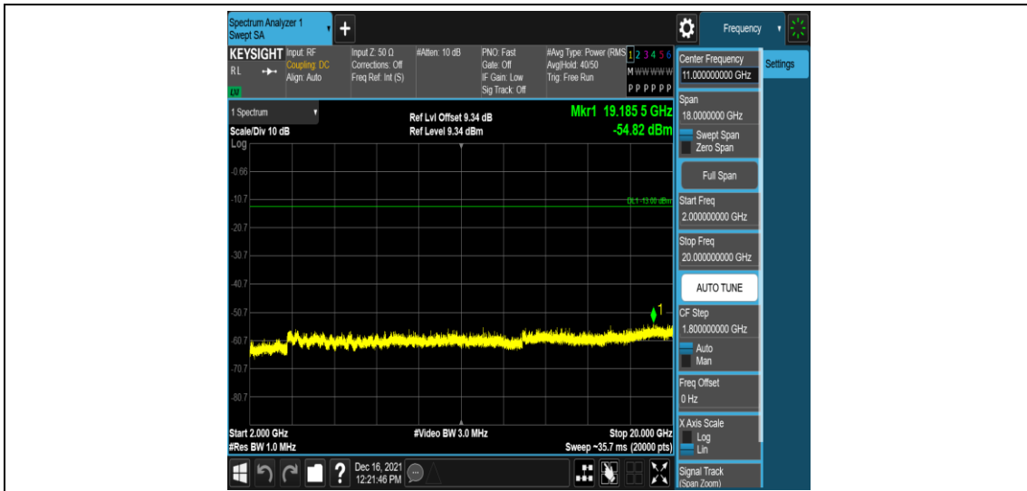
Band25-10MHz-16QAM-26090-1RB#0-Range5:2000~20000MHz
