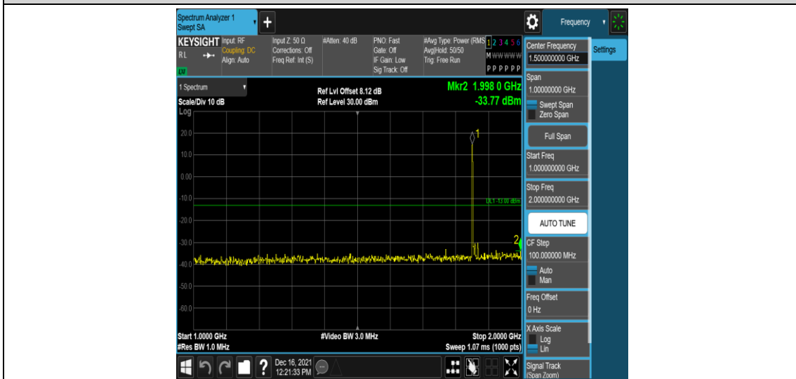
Band25-10MHz-16QAM-26090-1RB#0-Range4:1000~2000MHz
