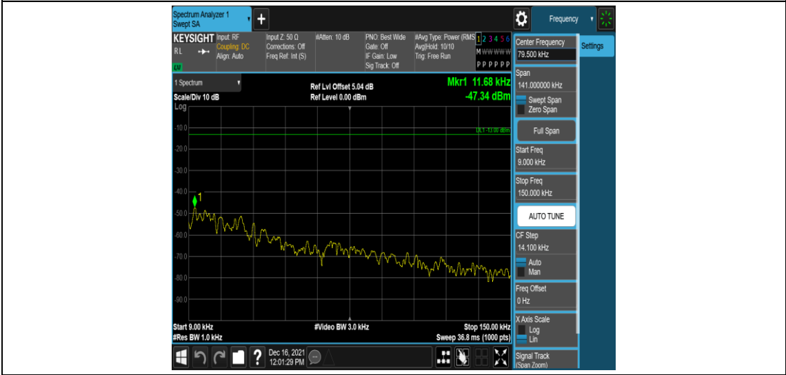
Band25-5MHz-QPSK-26365-1RB#0-Range1:0.009~0.15MHz
