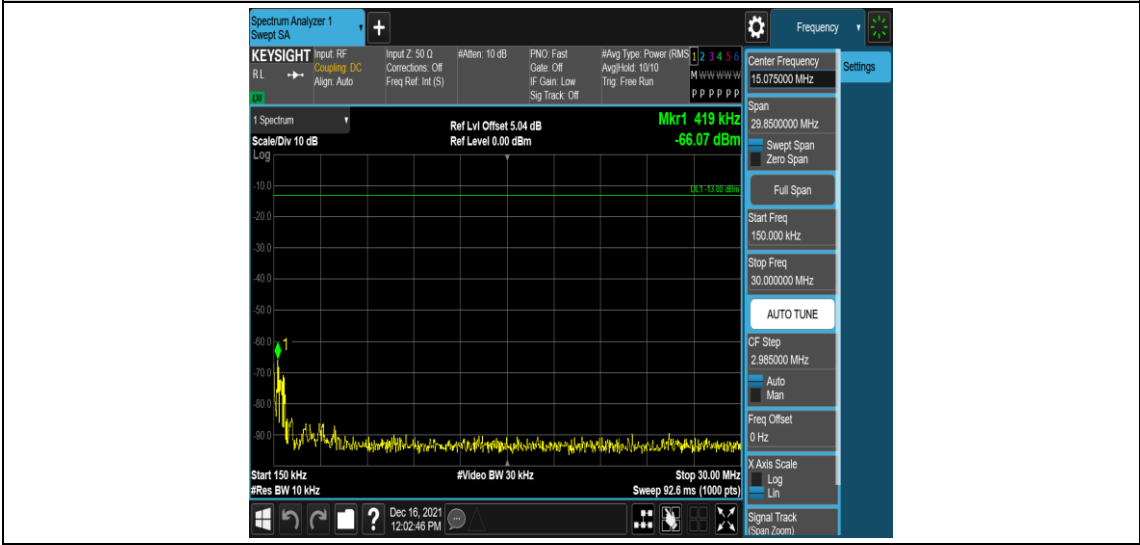
Band25-5MHz-16QAM-26365-1RB#0-Range2:0.15~30MHz
