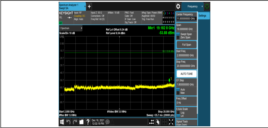
Band25-5MHz-QPSK-26365-1RB#0-Range5:2000~20000MHz
