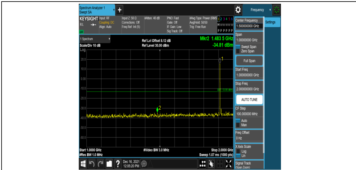
Band25-5MHz-16QAM-26665-1RB#0-Range4: 1000~2000MHz
