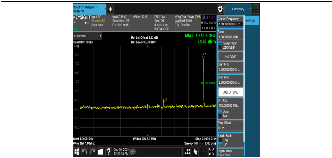
Band25-5MHz-QPSK-26665-1RB#0-Range4:1000~2000MHz
