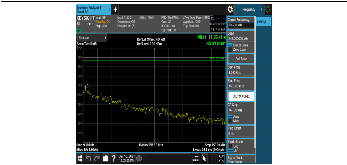
Band25-5MHz-QPSK-26665-1RB#0-Range1:0.009~0.15MHz
