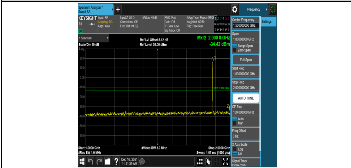
Band25-3MHz-16QAM-26365-1RB#0-Range4:1000~2000MHz
