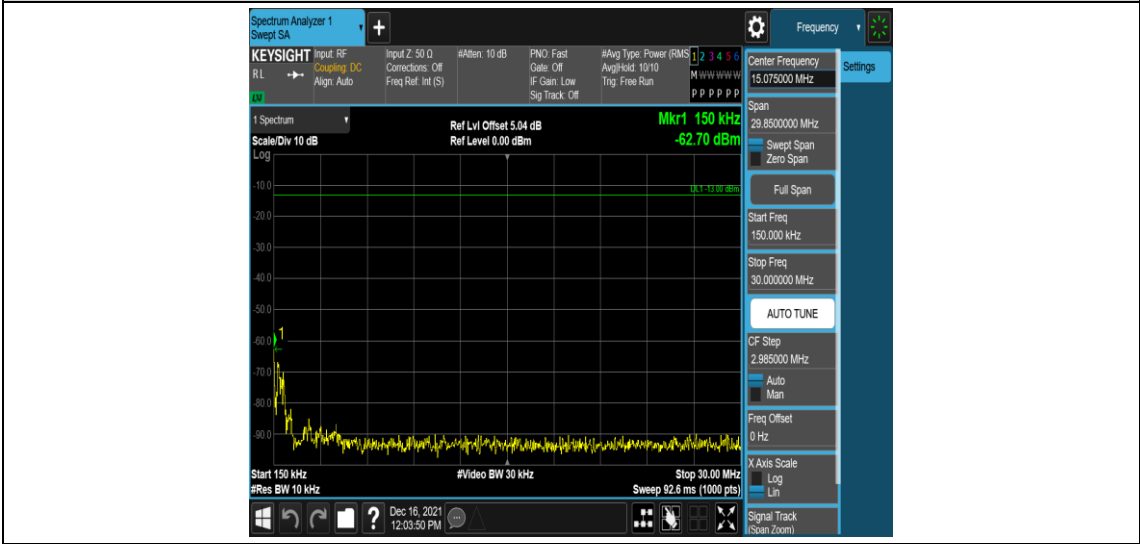
Band25-5MHz-QPSK-26665-1RB#0-Range2:0.15~30MHz
