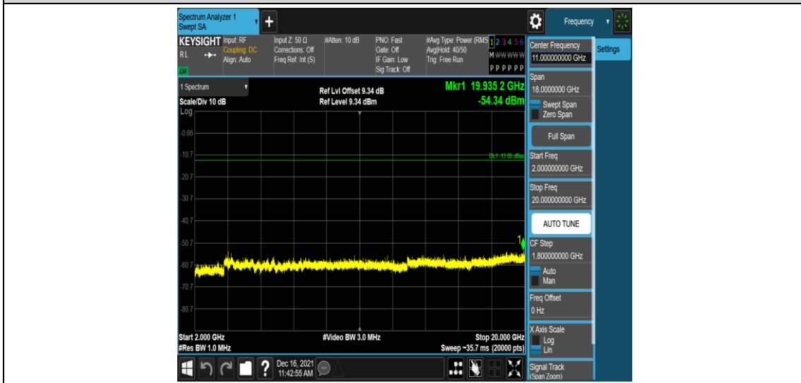
Band25-3MHz-QPSK-26675-1RB#0-Range5:2000~20000MHz
