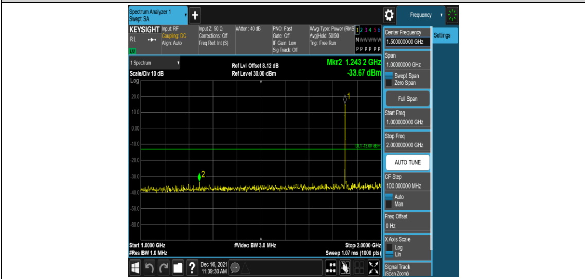
Band25-3MHz-16QAM-26055-1RB#0-Range4:1000~2000MHz
