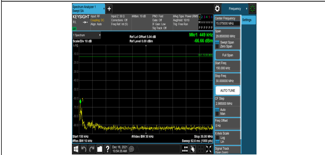
Band25-1.4MHz-16QAM-26683-1RB#0-Range2:0.15~30MHz
