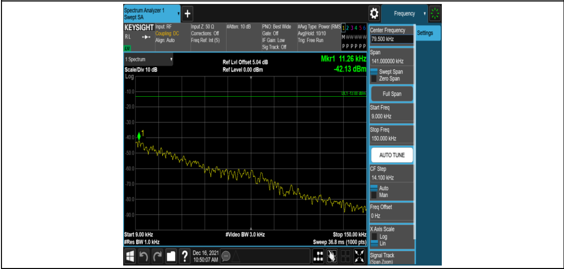
Band25-1.4MHz-16QAM-26047-1RB#0-Range1:0.009~0.15MHz
