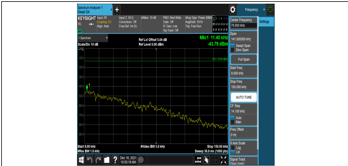
Band25-1.4MHz-QPSK-26683-1RB#0-Range1:0.009~0.15MHz
