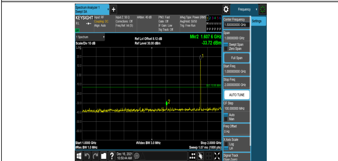
Band25-1.4MHz-16QAM-26047-1RB#0-Range4:1000~2000MHz
