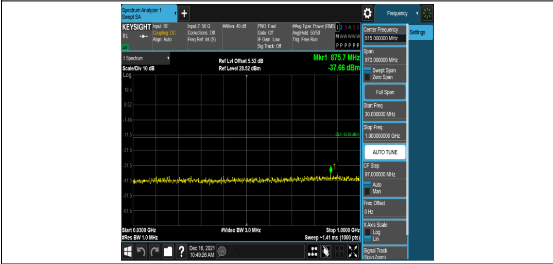
Band25-1.4MHz-QPSK-26047-1RB#0-Range3:30~1000MHz
