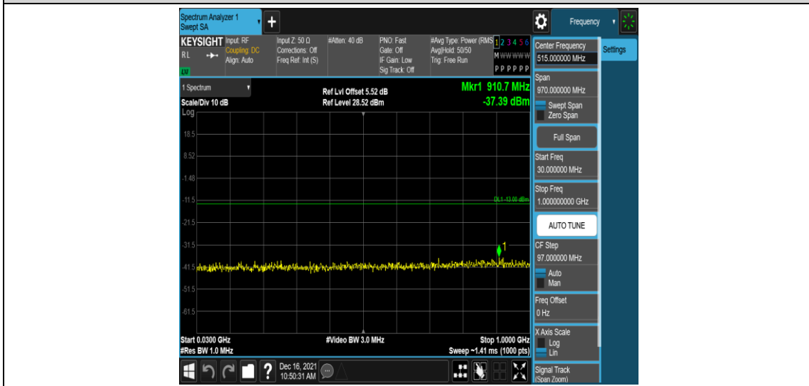
Band25-1.4MHz-16QAM-26047-1RB#0-Range3:30~1000MHz
