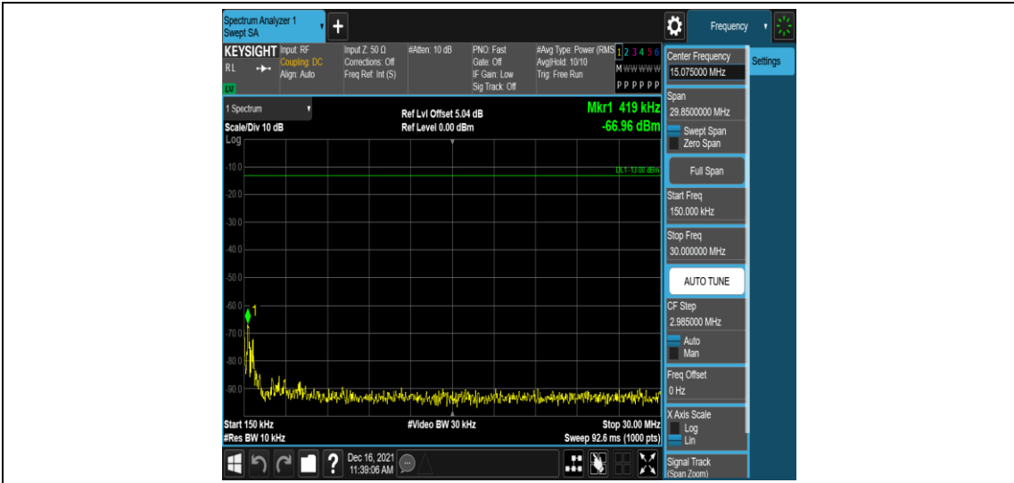
Band25-3MHz-16QAM-26055-1RB#0-Range2:0.15~30MHz
