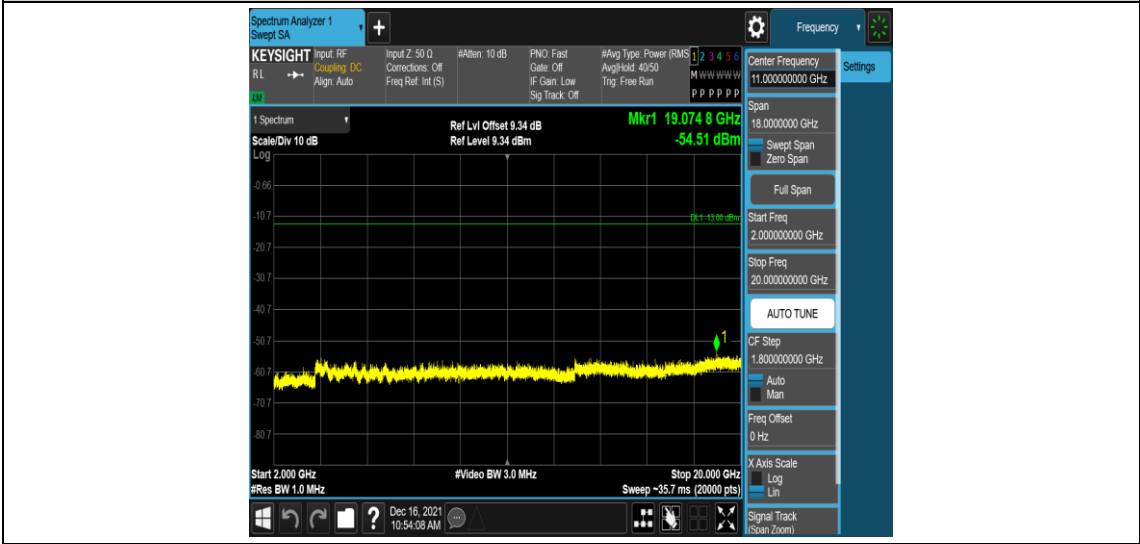
Band25-1.4MHz-QPSK-26683-1RB#0-Range5:2000~20000MHz
