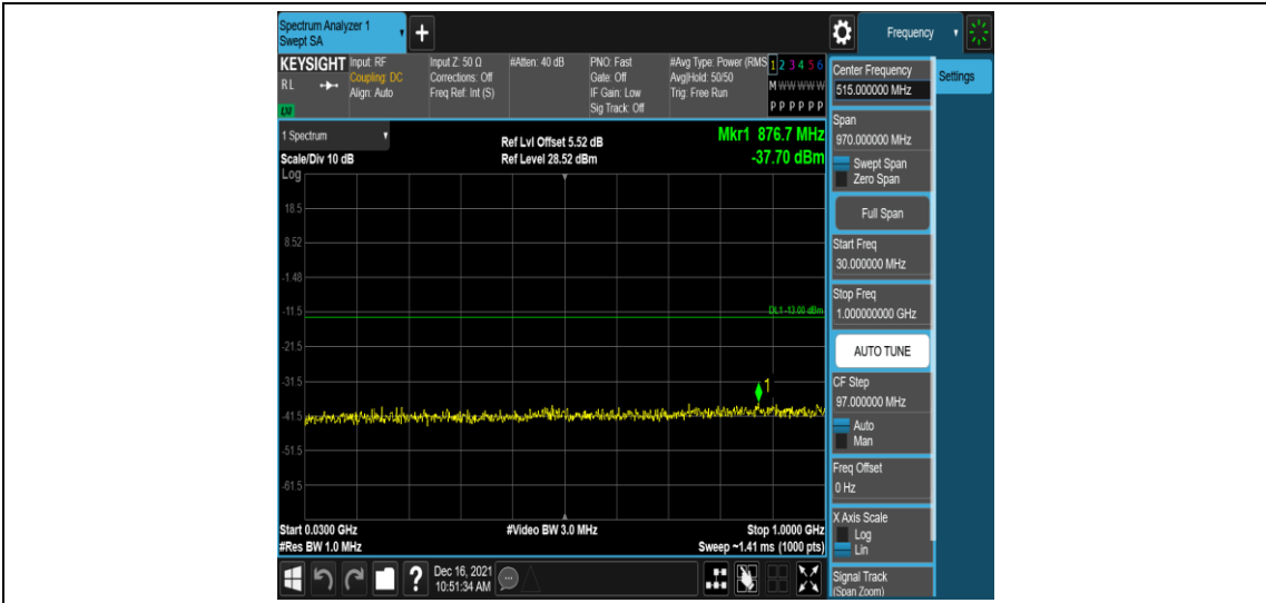
Band25-1.4MHz-QPSK-26365-1RB#0-Range3:30~1000MHz
