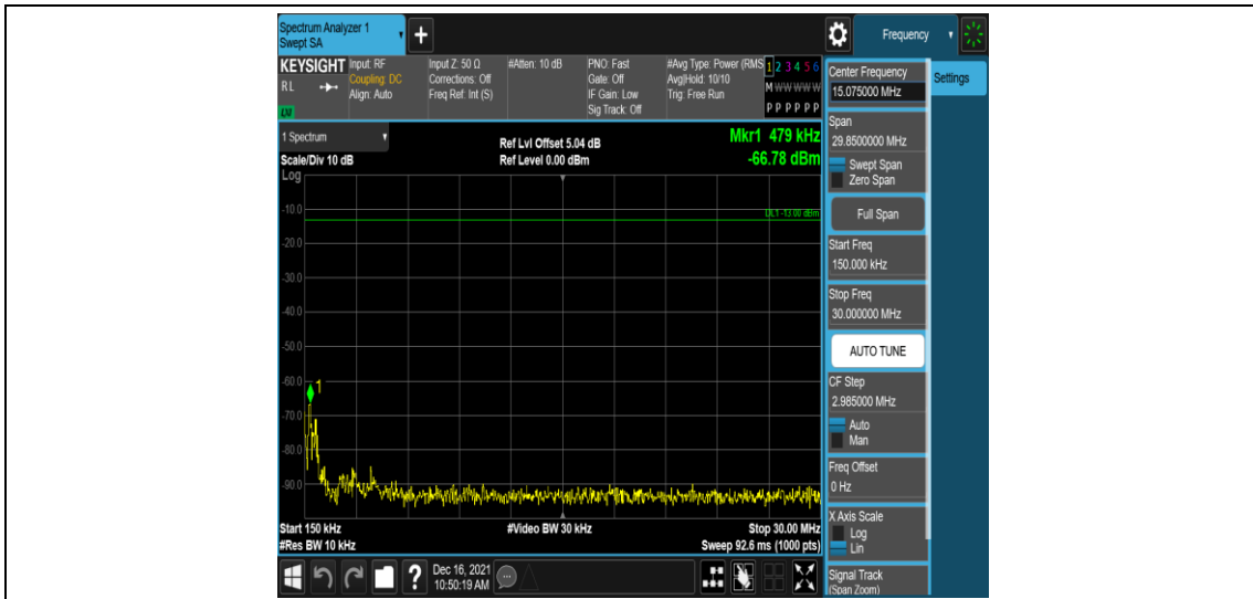
Band25-1.4MHz-16QAM-26047-1RB#0-Range2:0.15~30MHz
