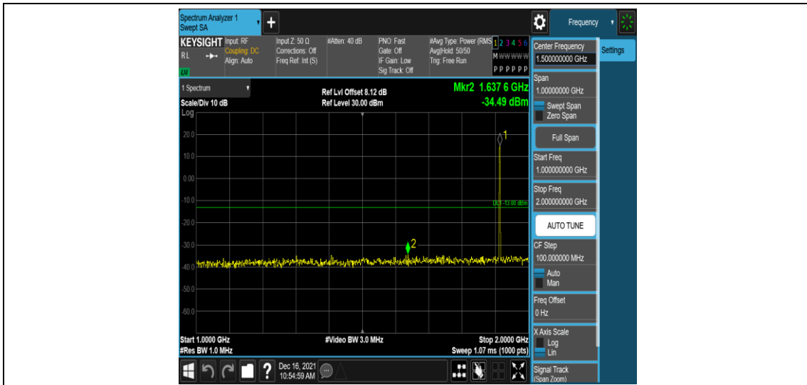
Band25-1.4MHz-16QAM-26683-1RB#0-Range4:1000~2000MHz
