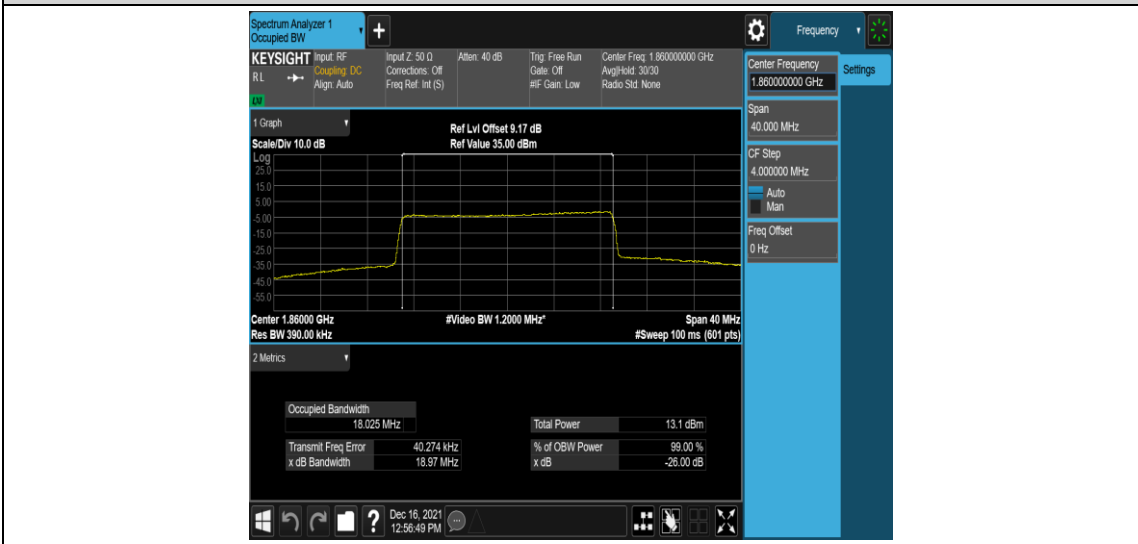
Band25-20MHz-QPSK-26140-100RB#0
