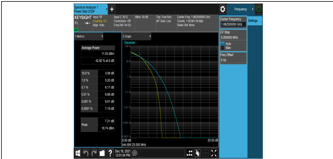
Band25-15MHz-16QAM-26365-75RB#0
