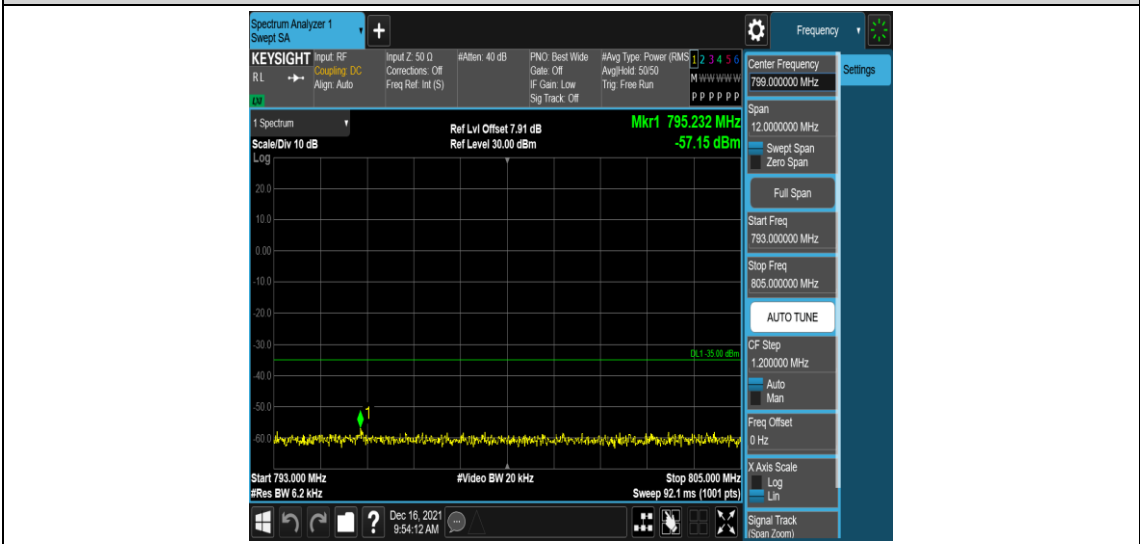
Band13-10MHz-16QAM-23230-1RB#0-Range6:793~805MHz
