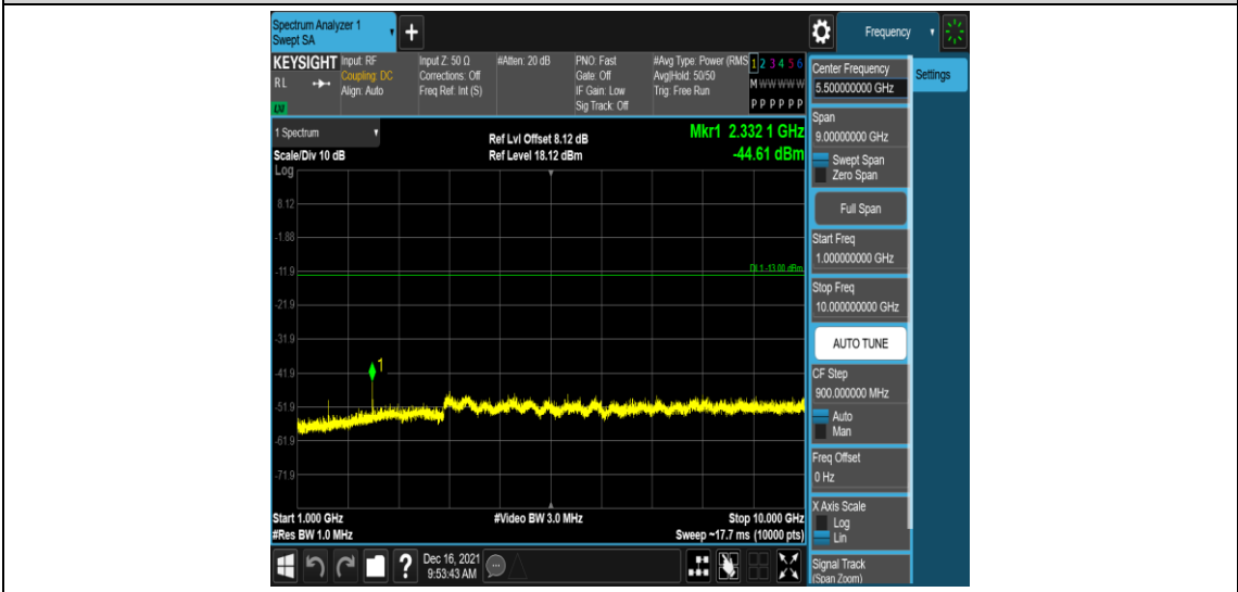
Band13-10MHz-16QAM-23230-1RB#0-Range4:1000~10000MHz
