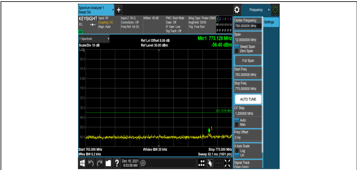
Band13-10MHz-16QAM-23230-1RB#0-Range5:763~775MHz
