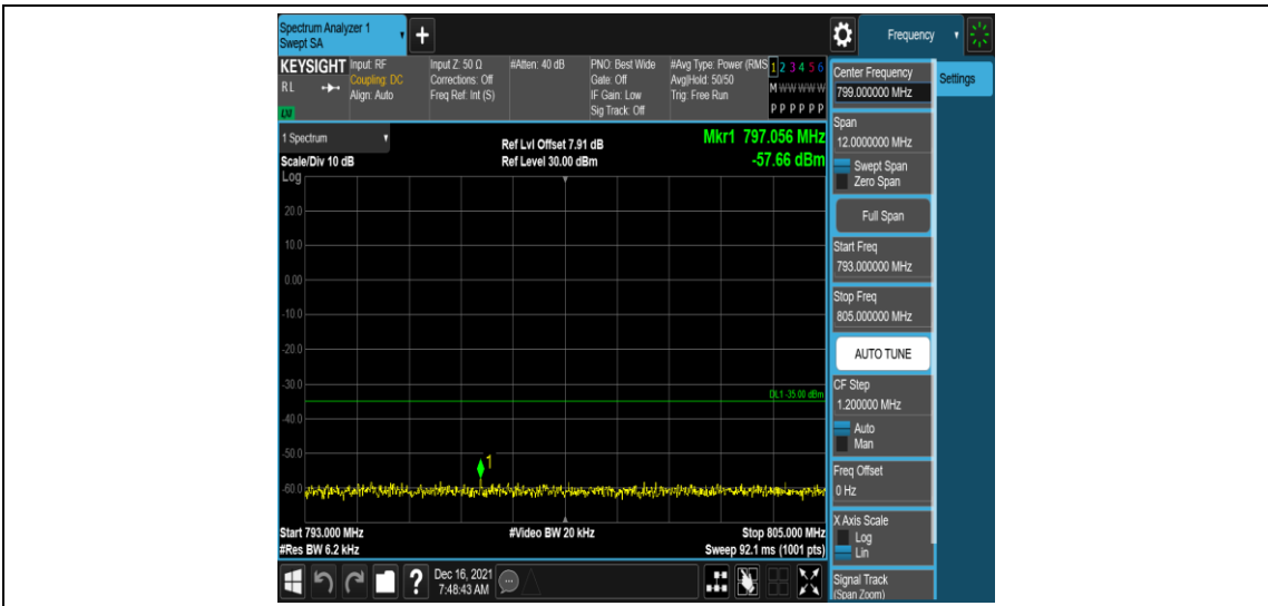
Band13-5MHz-QPSK-23205-1RB#0-Range6:793~805MHz
