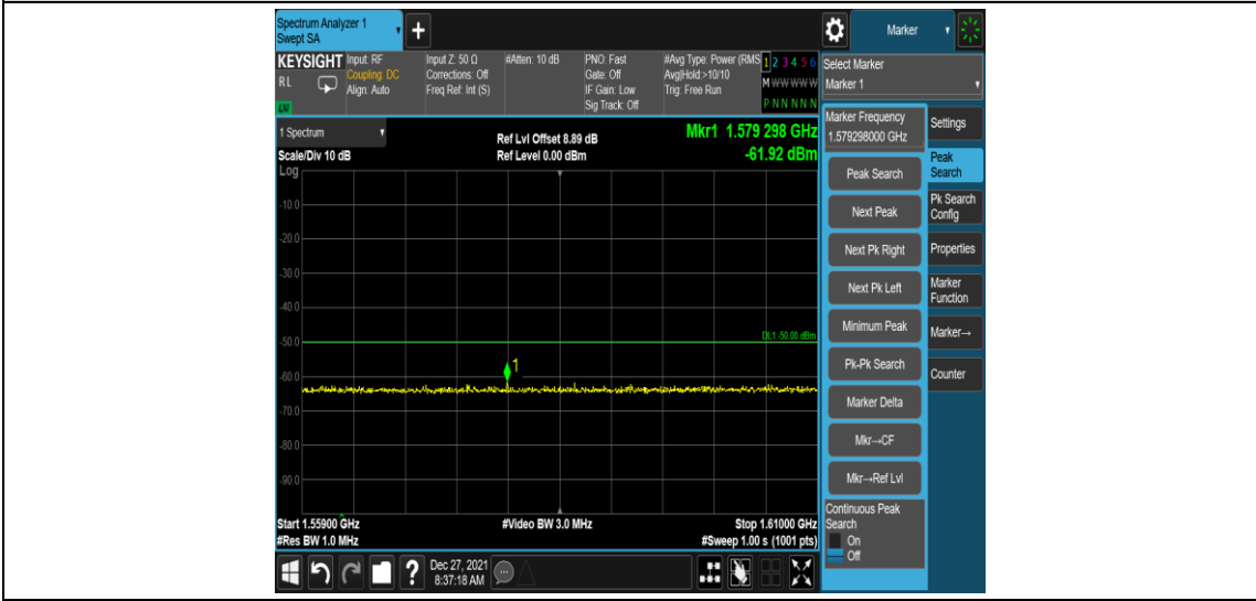
Band13-5MHz-QPSK-23205-1RB#0-Range7:1559~1610MHz
