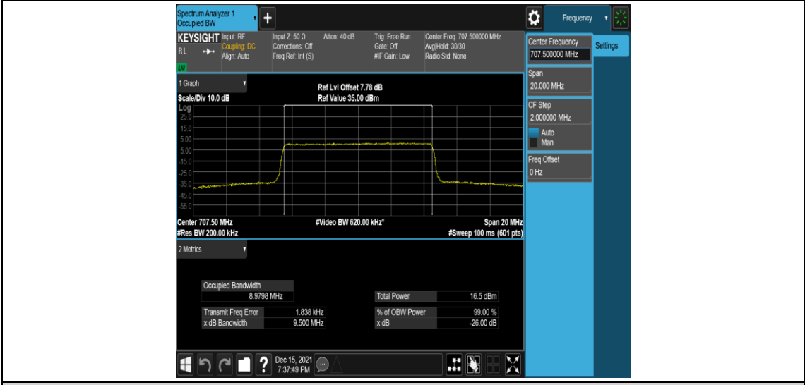
Band12-10MHz-16QAM-23095-50RB#0
