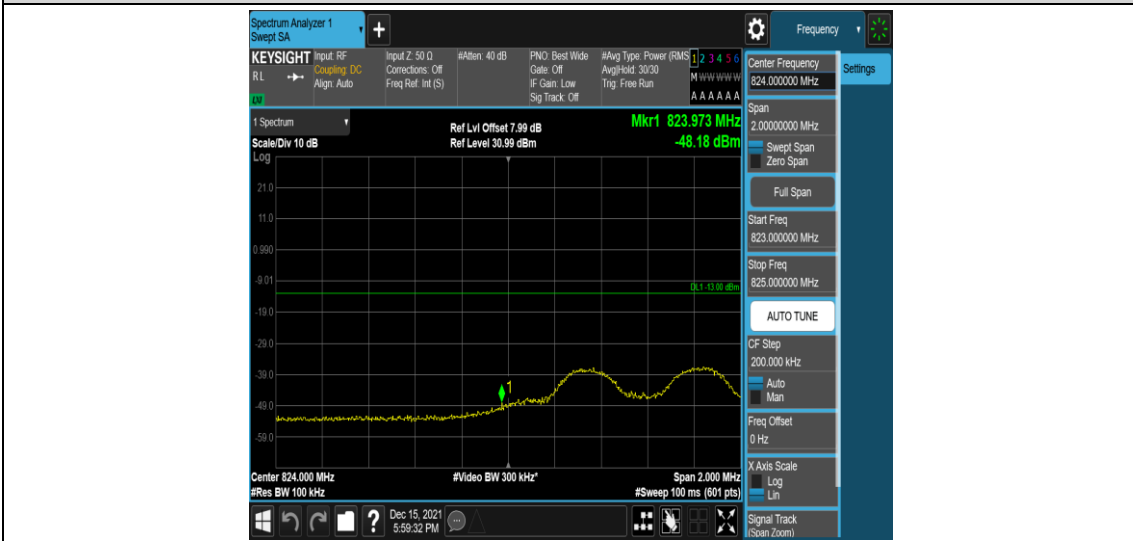
Band5-5MHz-16QAM-20425-1RB#24
