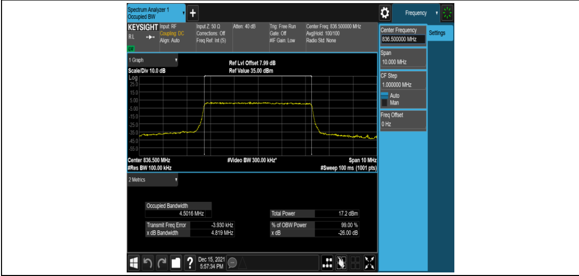
Band5-5MHz-16QAM-20525-25RB#0
