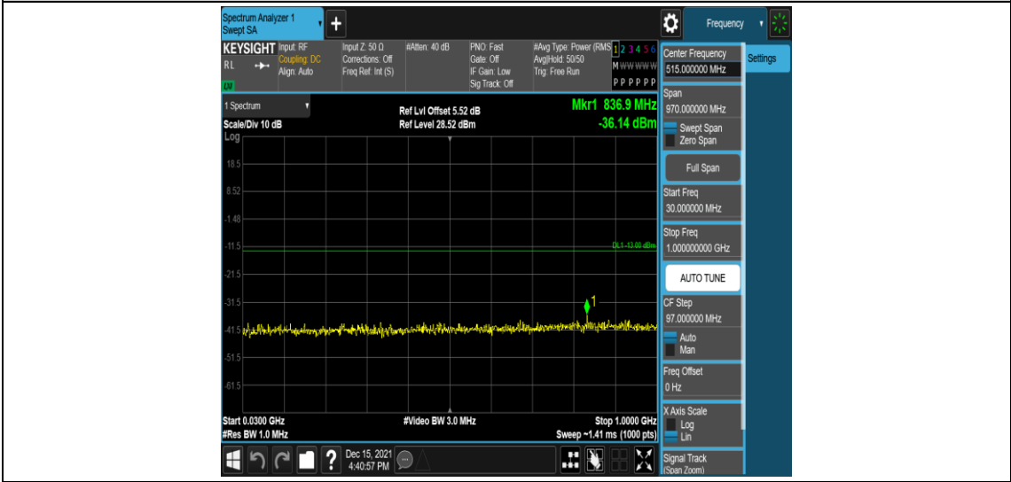
Band4-15MHz-QPSK-20025-1RB#0-Range3:30~1000MHz
