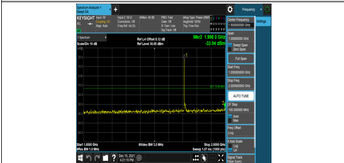
Band4-10MHz-16QAM-20000-1RB#0-Range4:1000~2000MHz
