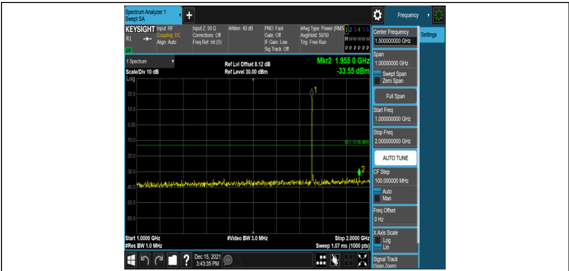
Band4-3MHz-16QAM-20385-1RB#0-Range4:1000~2000MHz
