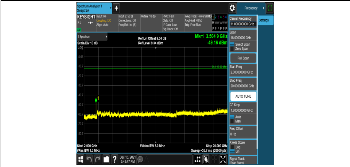
Band4-3MHz-16QAM-20385-1RB#0-Range5:2000~20000MHz
