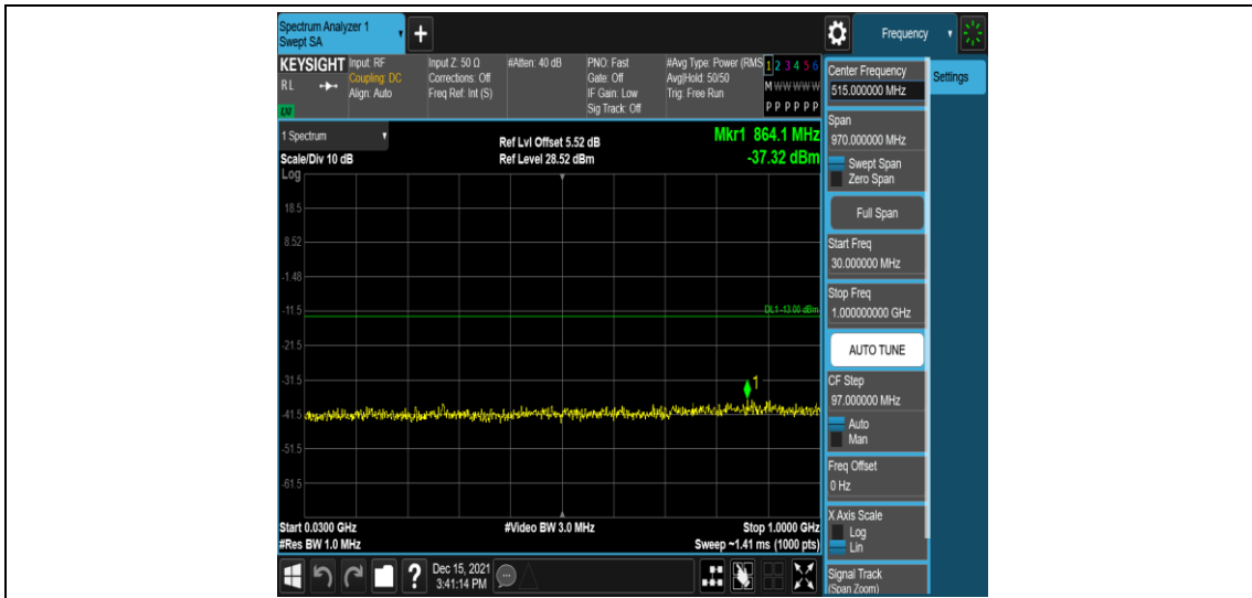
Band4-3MHz-16QAM-20175-1RB#0-Range3:30~1000MHz
