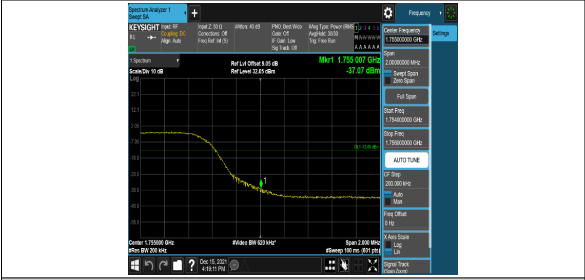
Band4-10MHz-16QAM-20350-50RB#0
