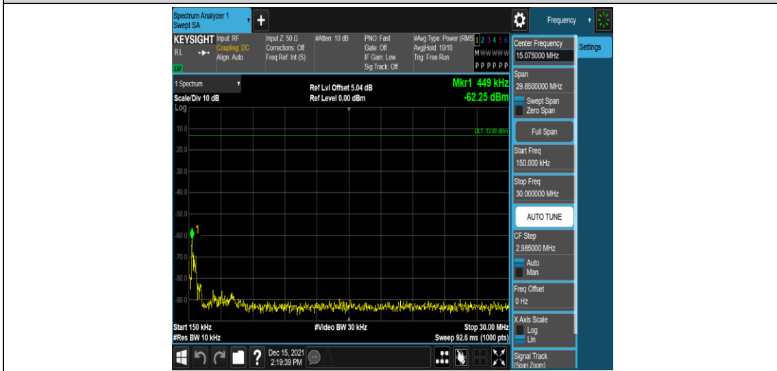
Band2-10MHz-16QAM-19150-1RB#0-Range2:0.15~30MHz
