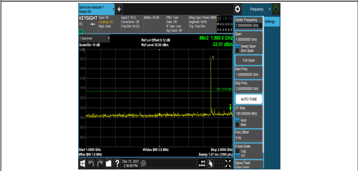
Band2-15MHz-16QAM-18675-1RB#0-Range4:1000~2000MHz
