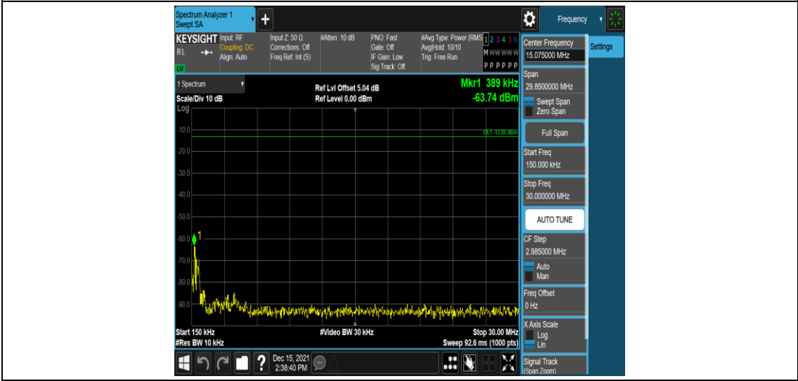
Band2-15MHz-16QAM-18900-1RB#0-Range2:0.15~30MHz
