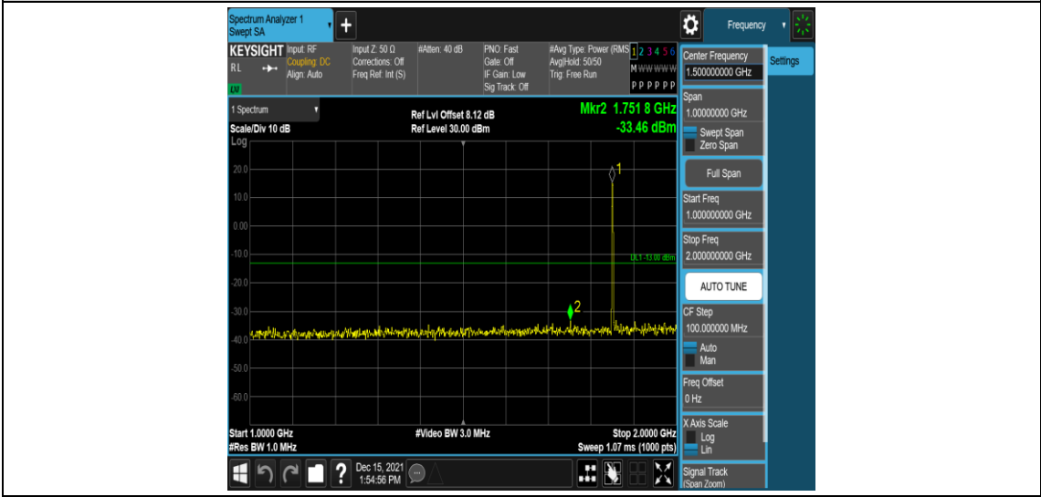
Band2-5MHz-16QAM-18625-1RB#0-Range4:1000~2000MHz
