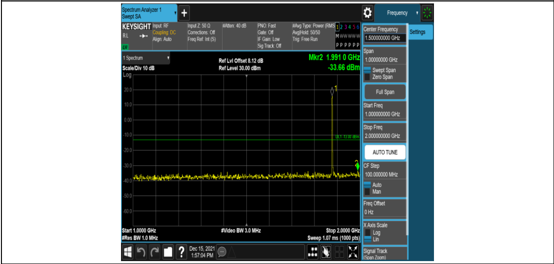
Band2-5MHz-16QAM-18900-1RB#0-Range4:1000~2000MHz
