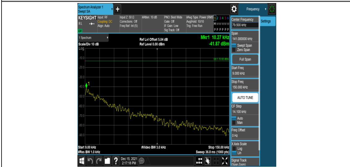
Band2-10MHz-16QAM-18900-1RB#0-Range1:0.009~0.15MHz
