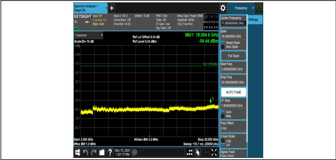
Band2-5MHz-16QAM-18900-1RB#0-Range5:2000~20000MHz
