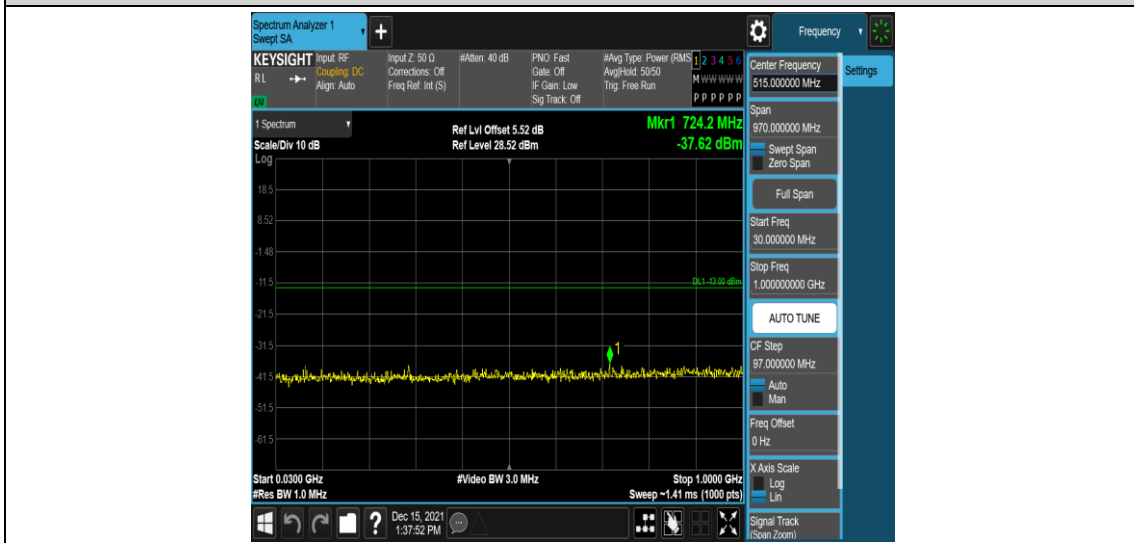
Band2-3MHz-16QAM-19185-1RB#0-Range3:30~1000MHz
