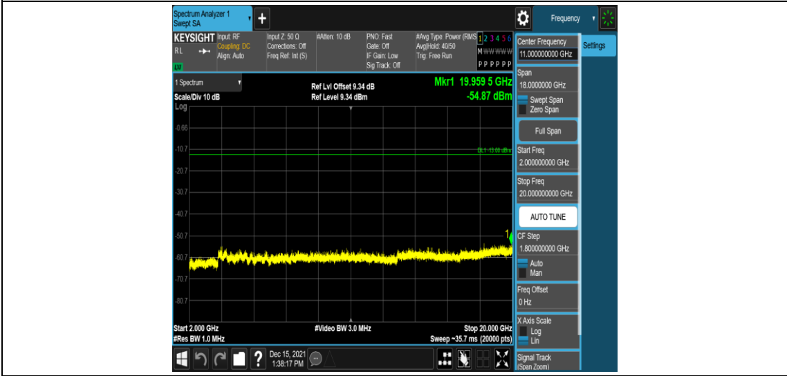
Band2-3MHz-16QAM-19185-1RB#0-Range5:2000~20000MHz
