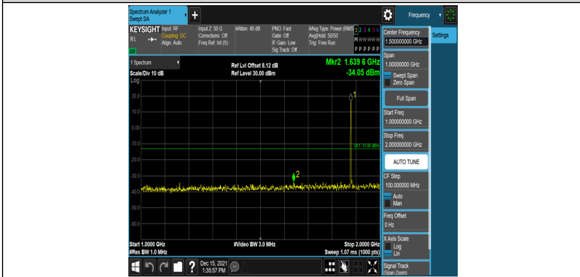
Band2-3MHz-16QAM-18900-1RB#0-Range4:1000~2000MHz
