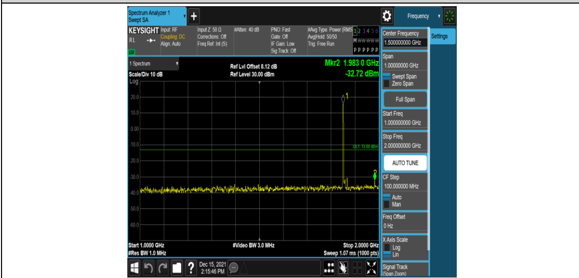
Band2-10MHz-16QAM-18650-1RB#0-Range4:1000~2000MHz
