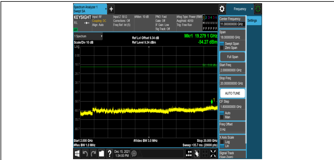
Band2-3MHz-16QAM-18615-1RB#0-Range5:2000~20000MHz
