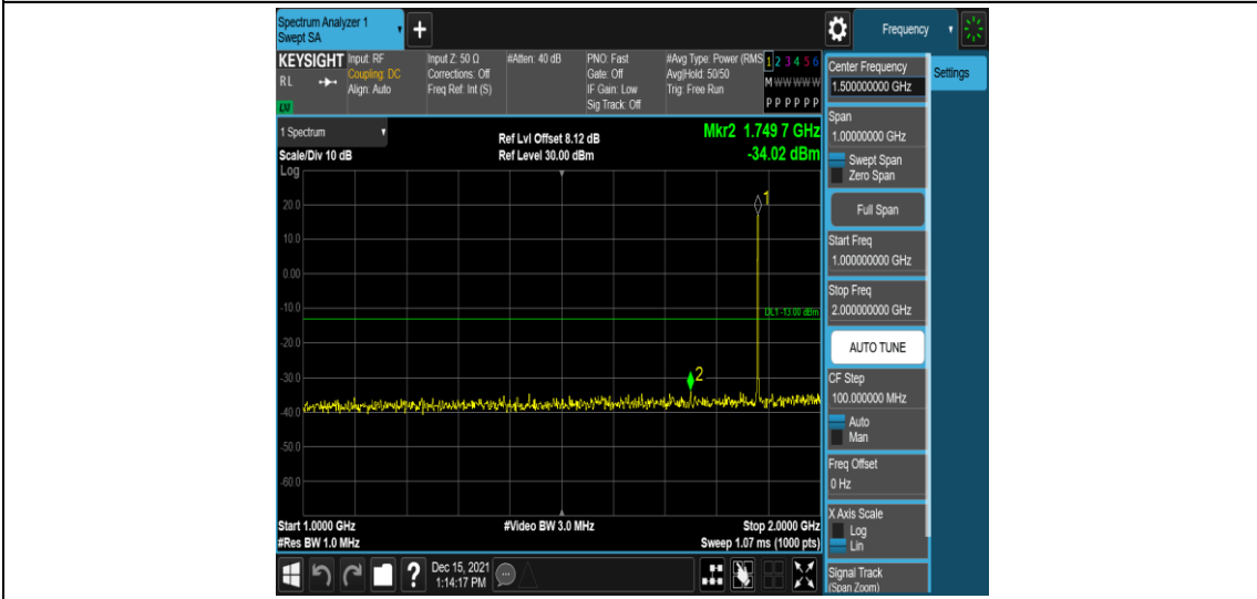
Band2-1.4MHz-QPSK-18900-1RB#0-Range4:1000~2000MHz
