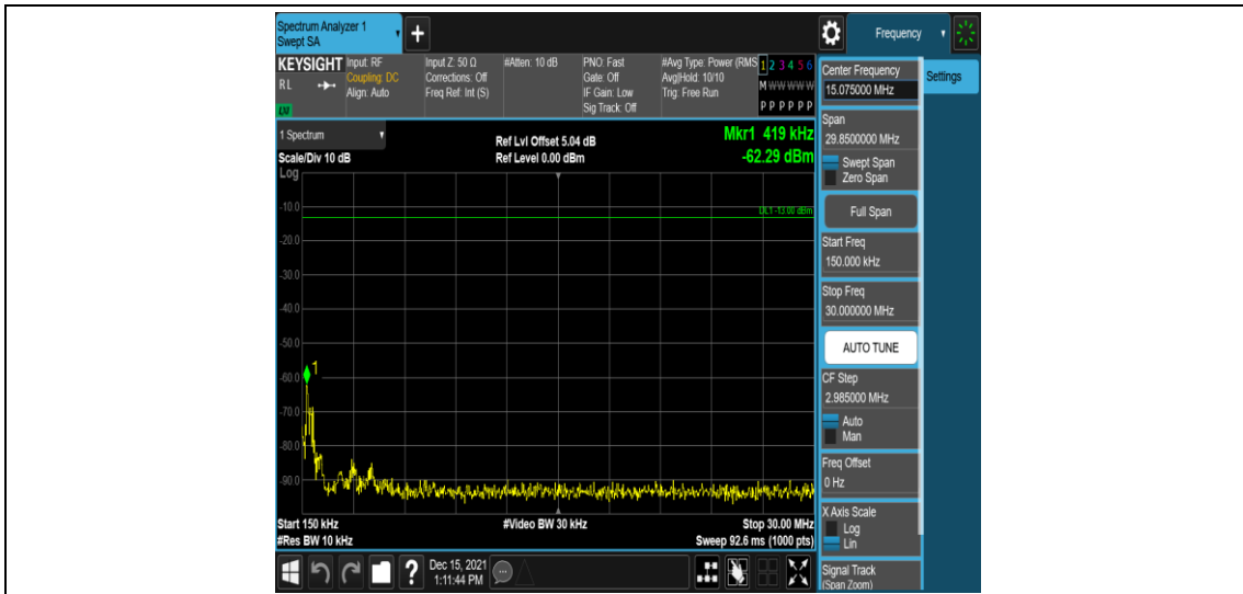
Band2-1.4MHz-QPSK-18607-1RB#0-Range2:0.15~30MHz
