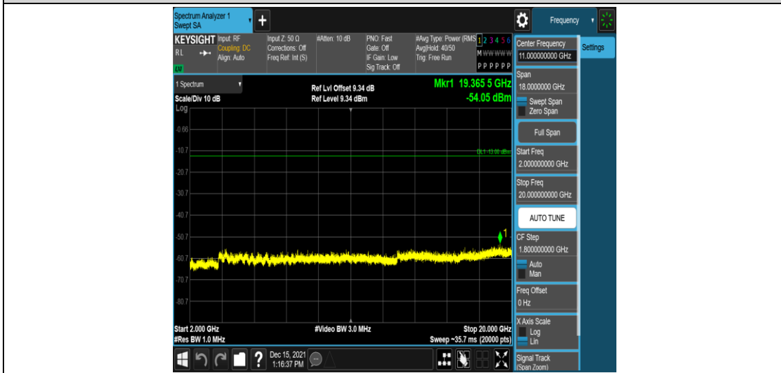
Band2-1.4MHz-QPSK-19193-1RB#0-Range5:2000~20000MHz
