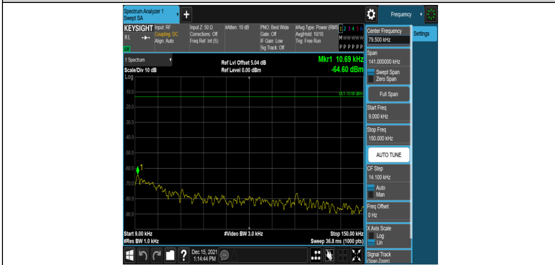
Band2-1.4MHz-16QAM-18900-1RB#0-Range1:0.009~0.15MHz
