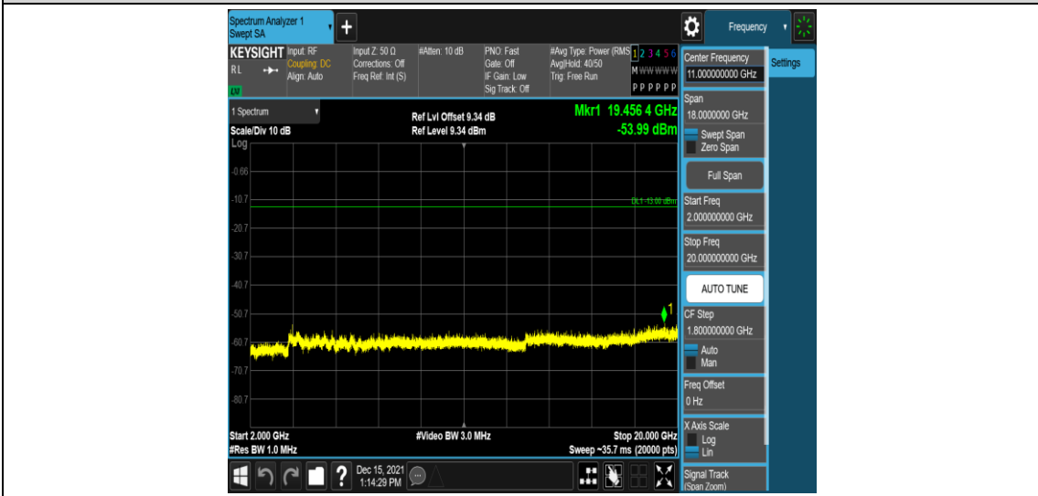
Band2-1.4MHz-QPSK-18900-1RB#0-Range5:2000~20000MHz
