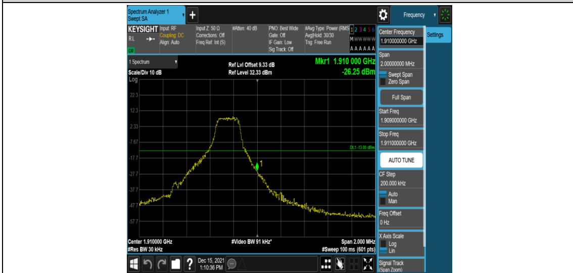
Band2-1.4MHz-16QAM-19193-1RB#5
