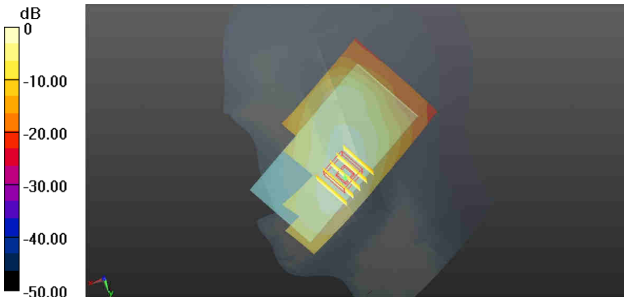
0 dB = 0.775 W/kg
