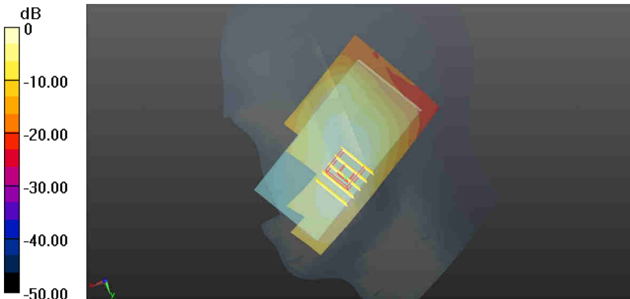
0 dB = 0.388 W/kg
