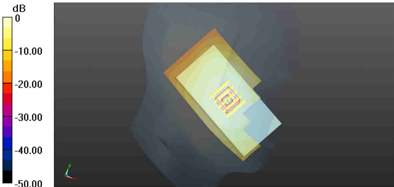
0 dB = 0.342 W/kg
