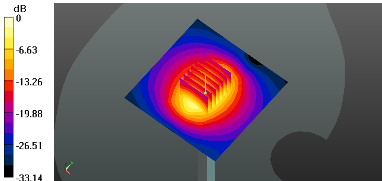
0 dB = 19.9 W/kg
