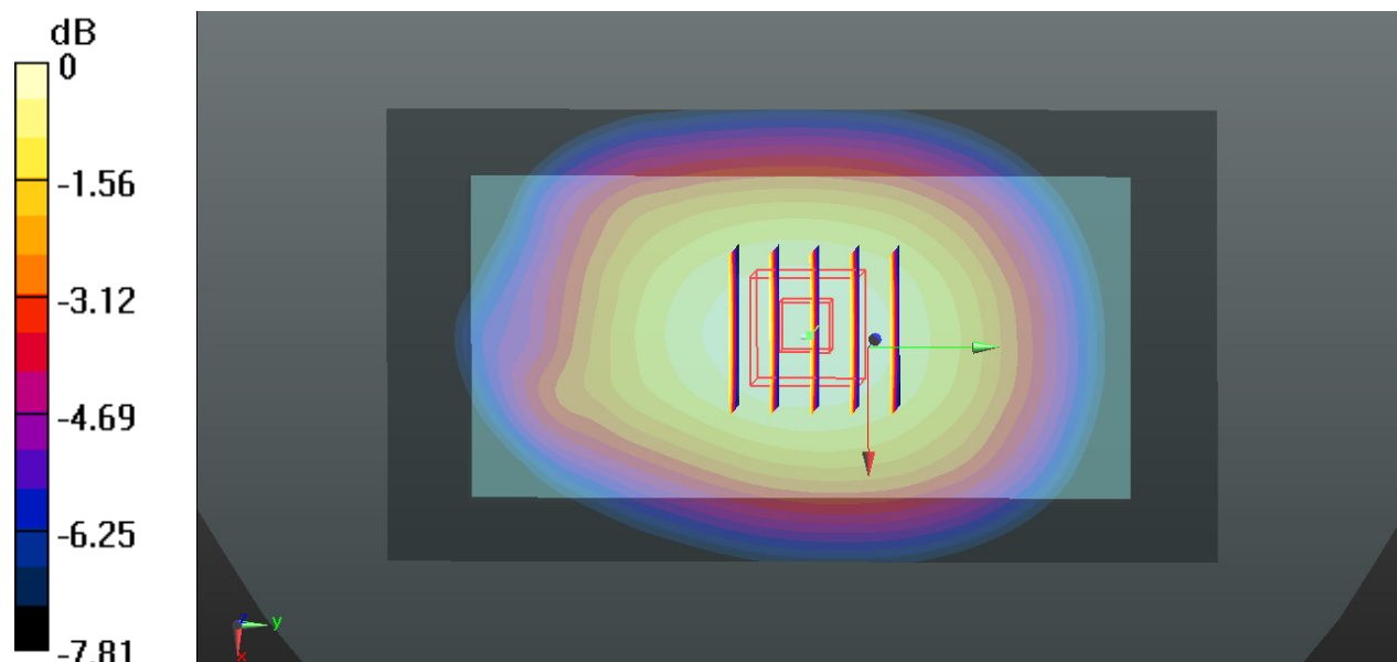
0 dB = 0.351 W/kg
