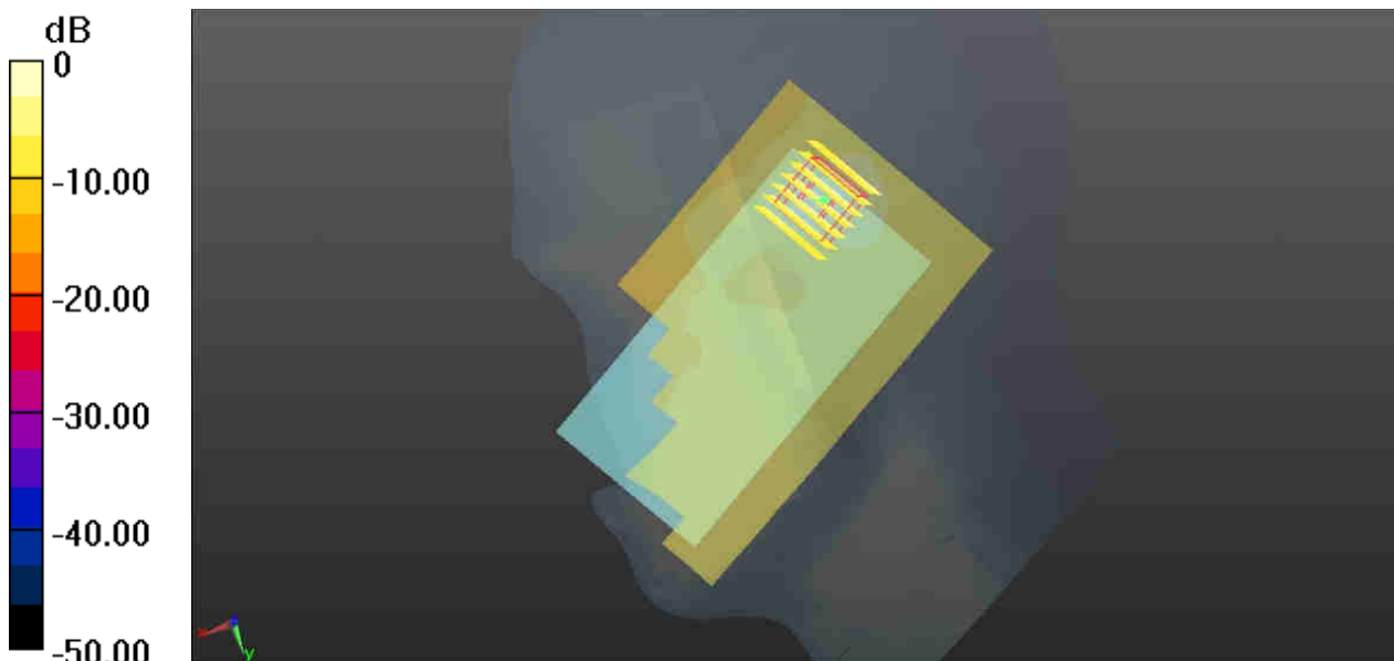
0 dB = 0.137 W/kg
