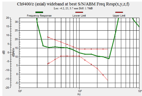
Fig 7.5 WCDMA Band II Ch9400
