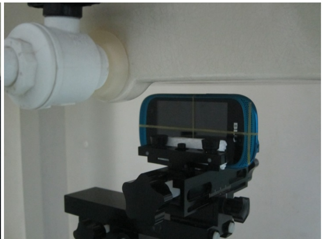
Left of the DUT with Phantom 1 cm Gap
