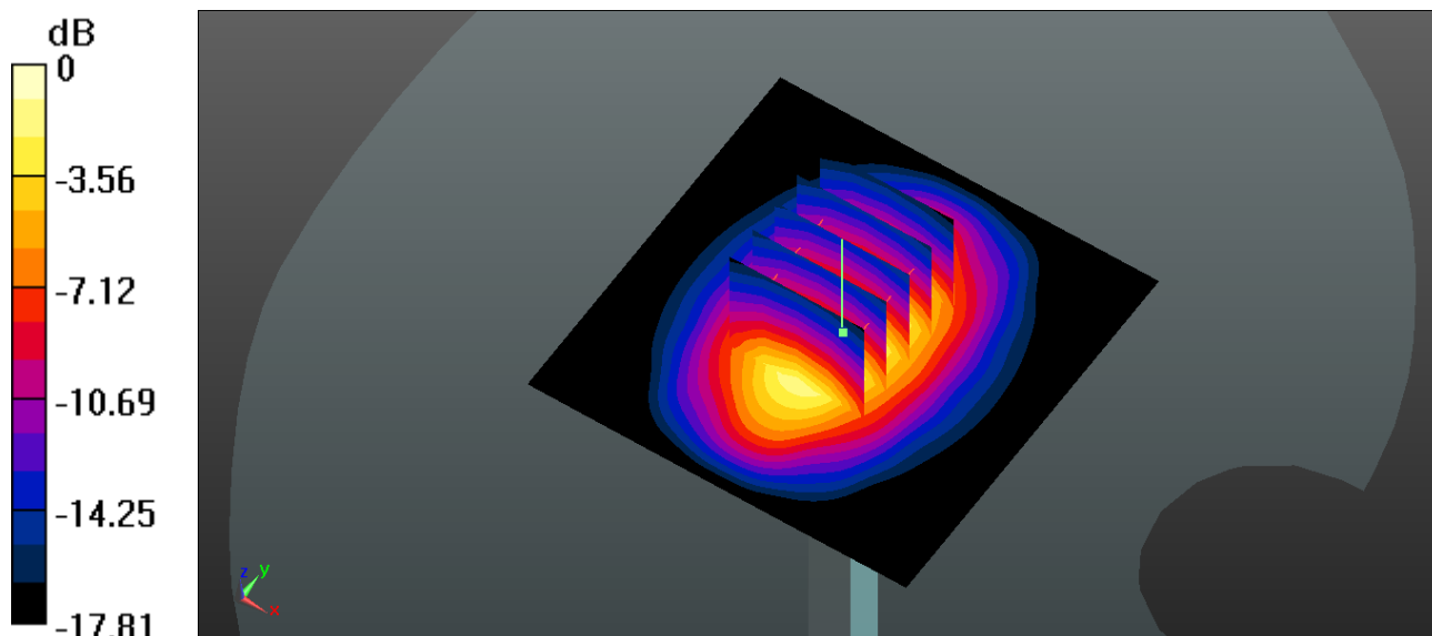
0 dB = 17.2 W/kg
