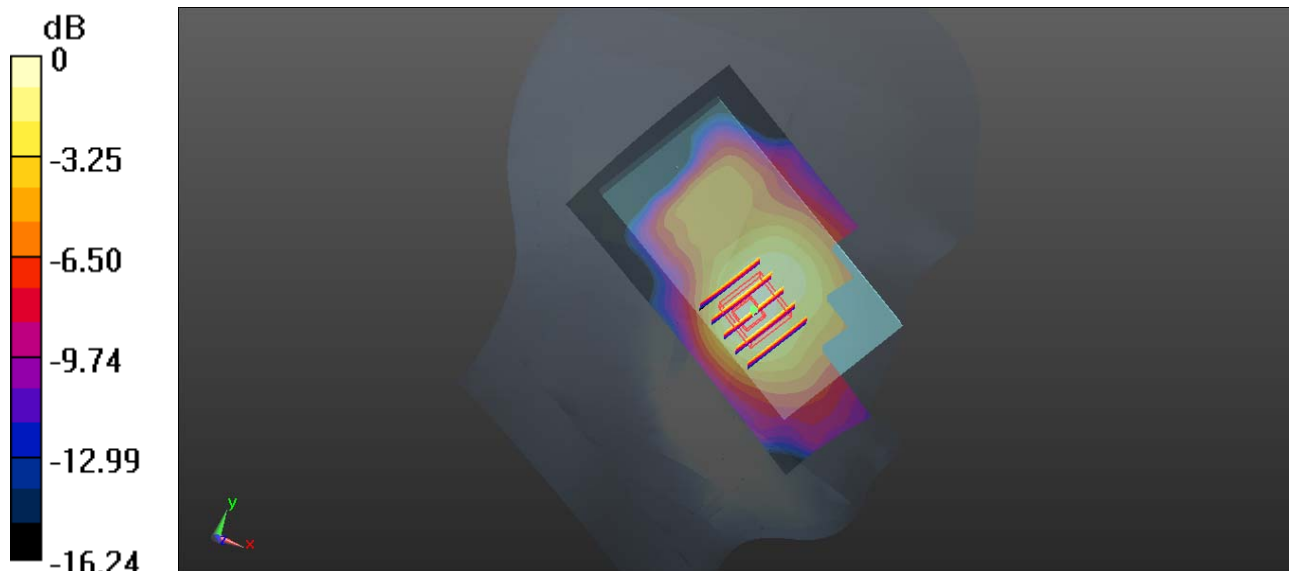
0 dB = 0.650 W/kg
