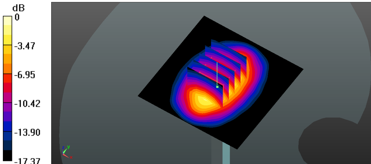
0 dB = 16.3 W/kg
