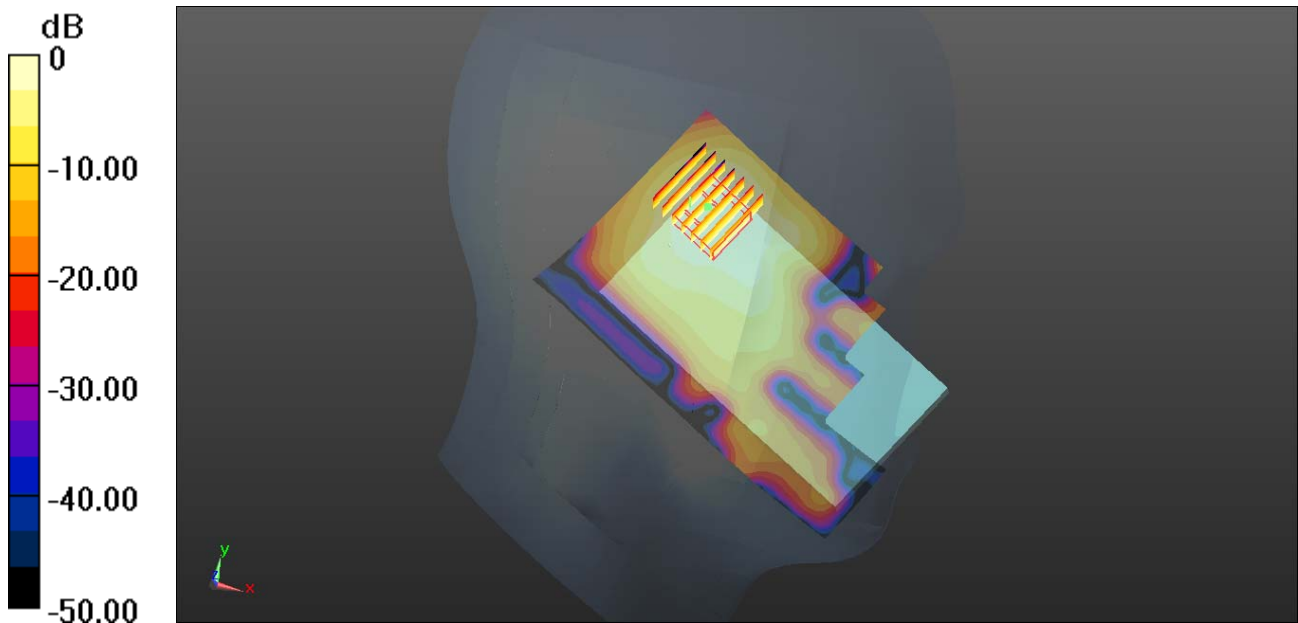
0 dB = 0.378 W/kg
