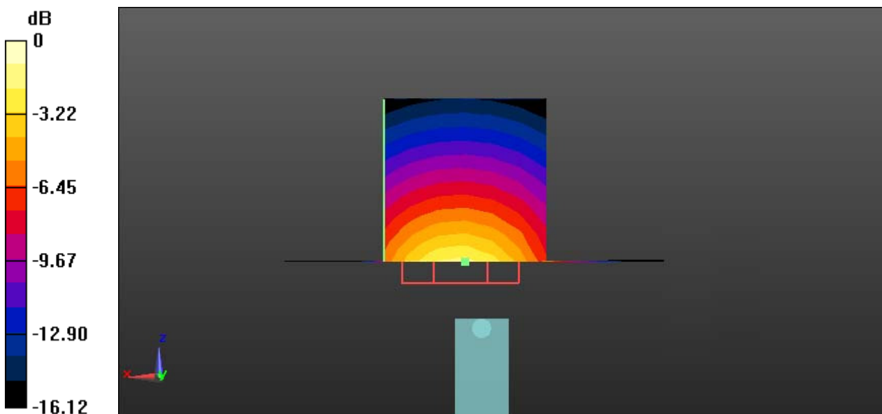
0 dB = 41.2 W/kg = 16.15 dBW/kg
