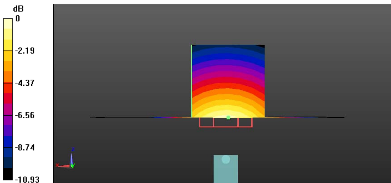
0 dB = 10.8 W/kg = 10.33 dBW/kg
