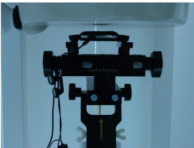
Back of DUT with Earphone to Phantom 1 cm Gap
