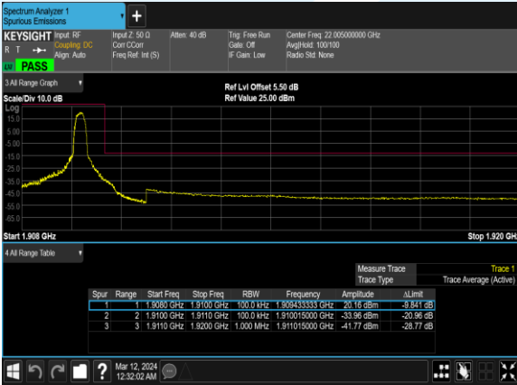
B2_10M_16QAM_1@49_CH_19150
