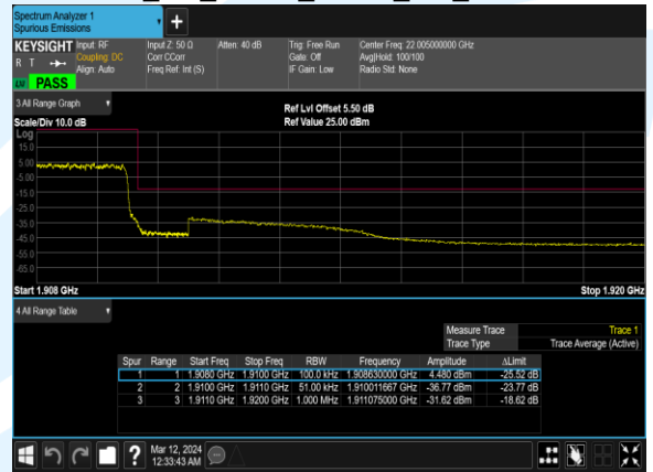
B2_5M_16QAM_25@0_CH_19175
