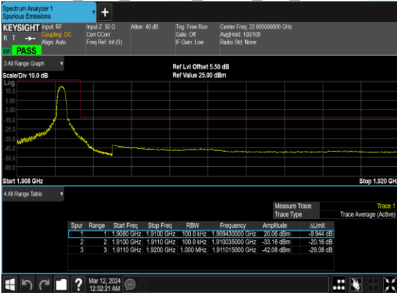
B2_10M_16QAM_1@49_CH_19150
