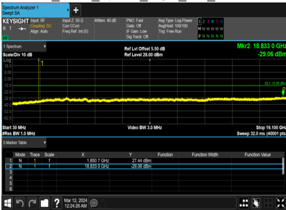
B2_1.4M_QPSK_1@0_CH_18900
