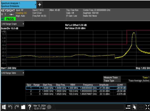
B2_10M_16QAM_1@0_CH_18650
