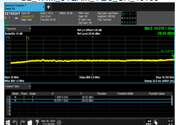
B2_1.4M_64QAM_1@0_CH_19193
