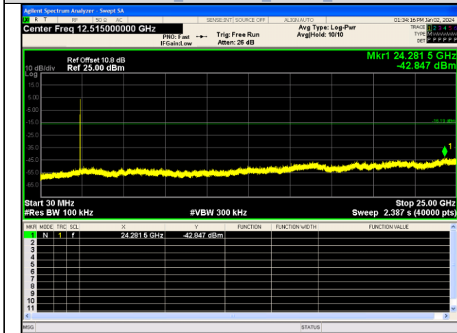
Spurion Emission IEEE 802.11b Channel 1 20MHz Antenna 0
