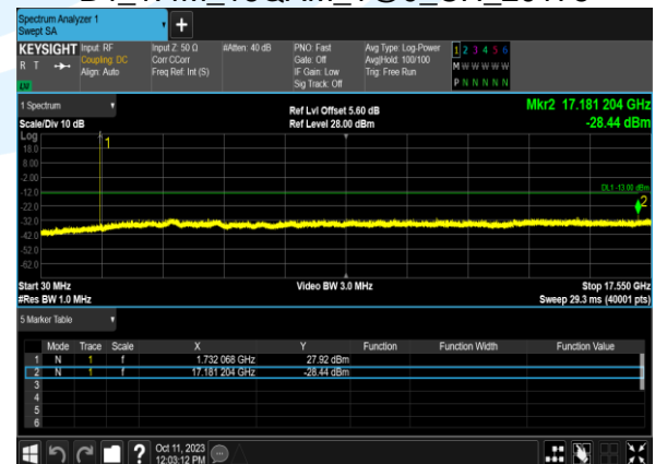
B4_1.4M_16QAM_1@0_CH_20175
