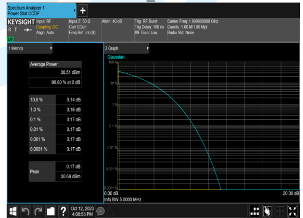
GPRS1900_Channel810
