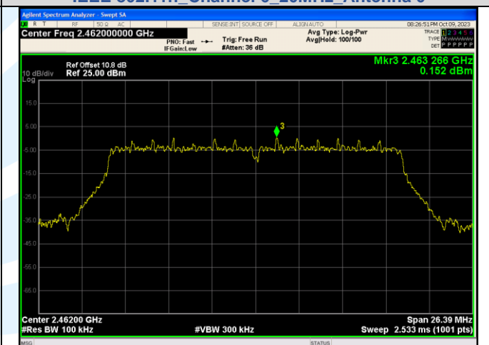
In-Band Reference Level IEEE 802.11n_Channel 11_20MHz_Antenna 0
