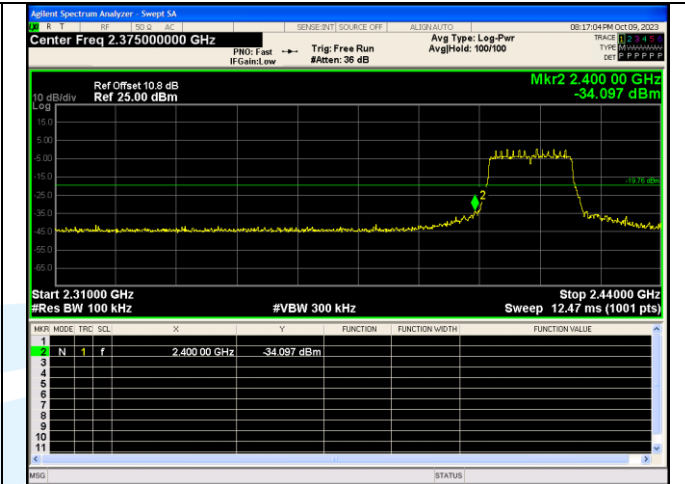
Out Of Band Emission IEEE 802.11n_Channel 1_20MHz_Antenna 0
