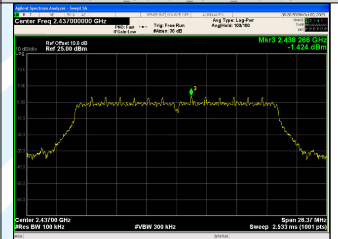
In-Band Reference Level IEEE 802.11n_Channel 6_20MHz_Antenna 0
