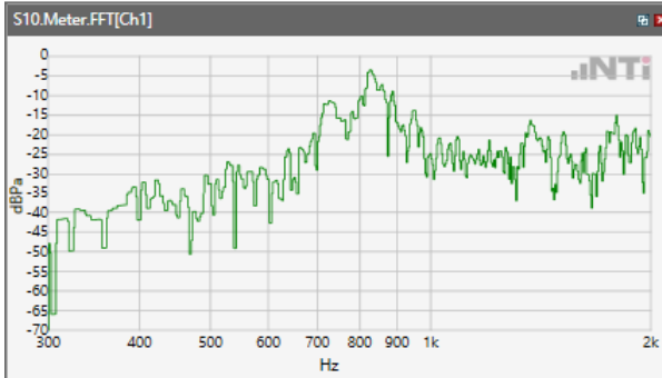
ANSI/TIA 5050-2018 \ 8N HAC OFF \ NB 12.2kbps\ 5.2 Receive path – distortion and noise\WLAN 5.8 GHz
