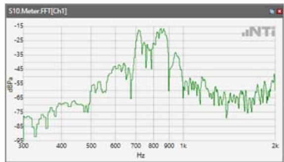
ANSI/TIA 5050-2018 \ 8N HAC OFF \ NB 12.2kbps\ 5.2 Receive path – distortion and noise\ LTE Band 25
