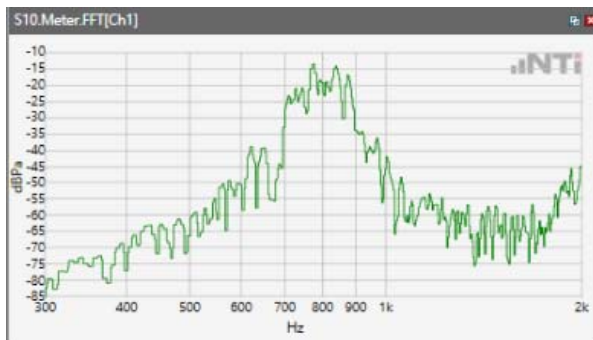
ANSI/TIA 5050-2018 \ 8N HAC OFF \ NB 12.2kbps\ 5.2 Receive path – distortion and noise\LTE Band 26
