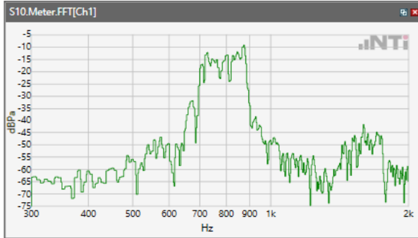
ANSI/TIA 5050-2018 \ 8N HAC OFF \ NB 12.2kbps\ 5.2 Receive path – distortion and noise\WLAN 5.2 GHz
