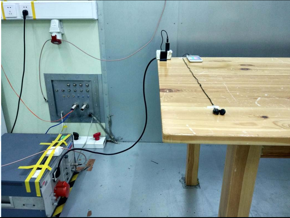
Conducted Emission Test Setup - Mode 4
