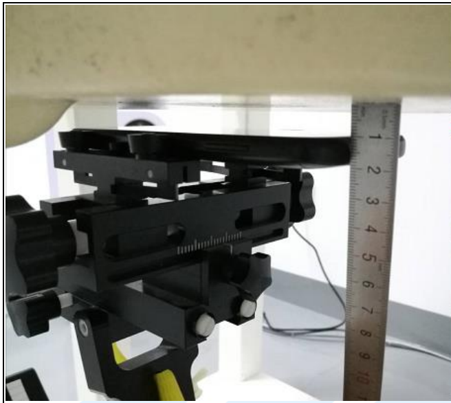
Front Face of EUT with 1.0 cm Gap
