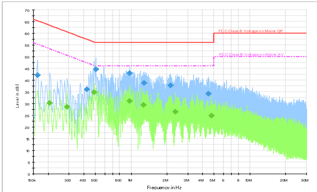
Fig.B.9.3 AC Powerline Conducted Emission- Bluetooth, charger TN-050120U8
