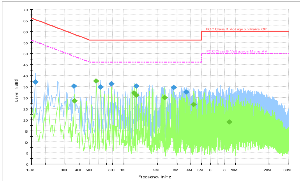
Fig.B.9.1 AC Powerline Conducted Emission- Bluetooth, charger TN-050120U9
