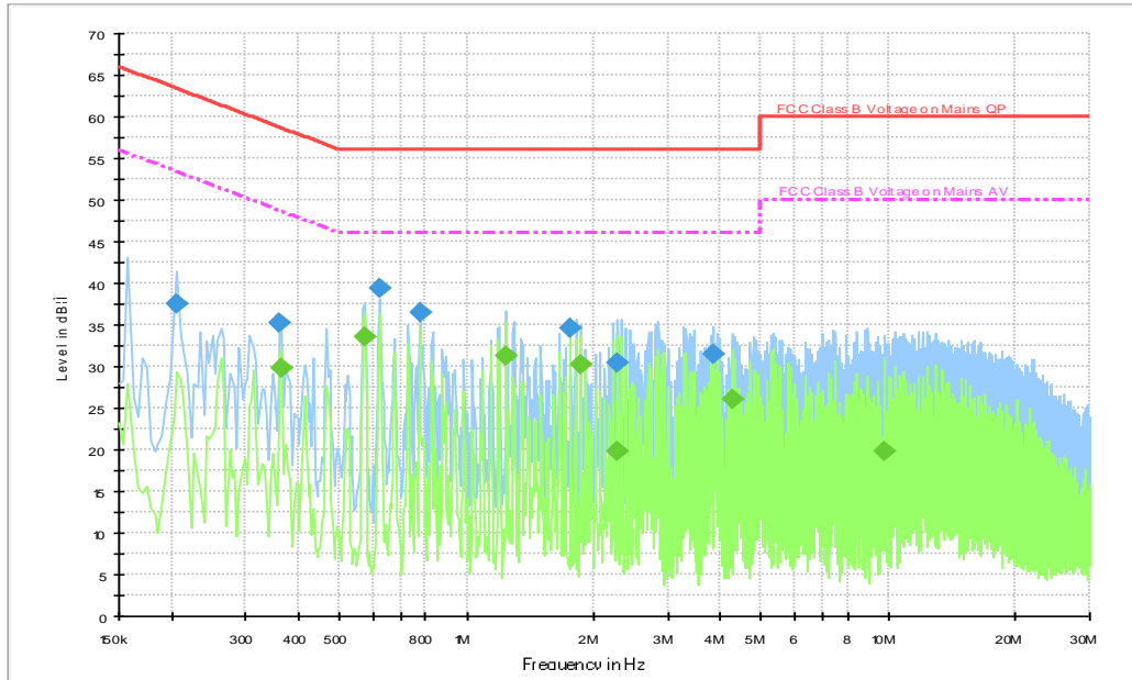
Fig.B.9.2 AC Powerline Conducted Emission-Idle, charger TN-050120U9
